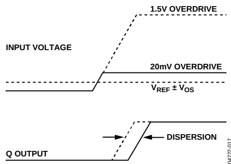
Figure 18. Propagation Delay Dispersion
