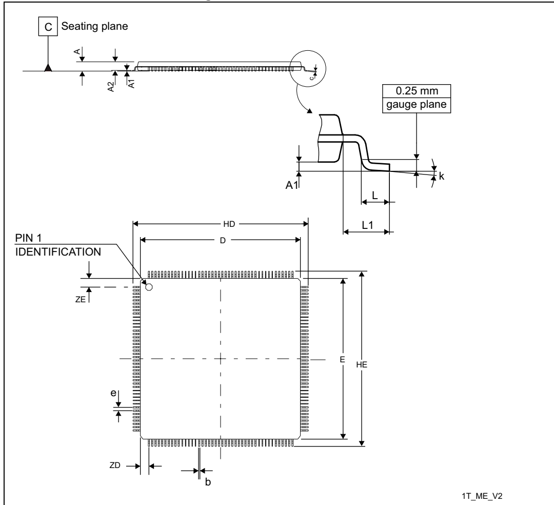
Figure 88. LQFP176 outline
