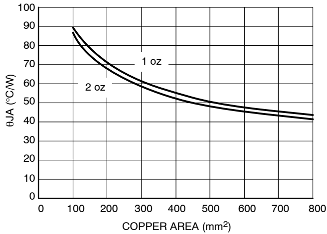
Figure 21. D²PAK 7-lead \theta_{JA} as a Function of the Pad Copper Area Including Traces, Board Material
