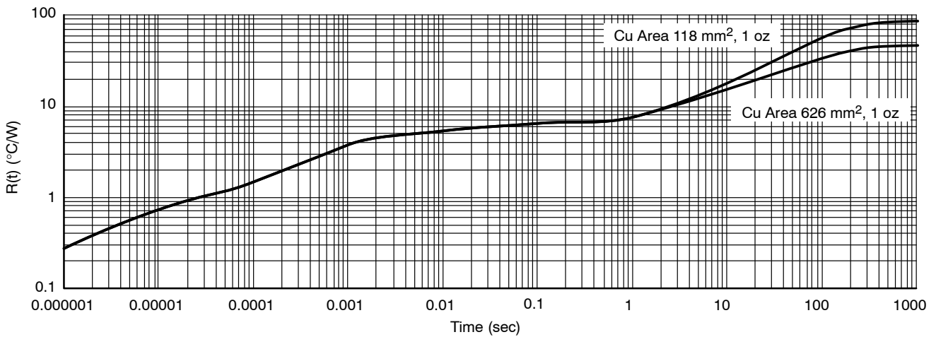
Figure 22. D²PAK 7-Lead Single Pulse Heating Curve
