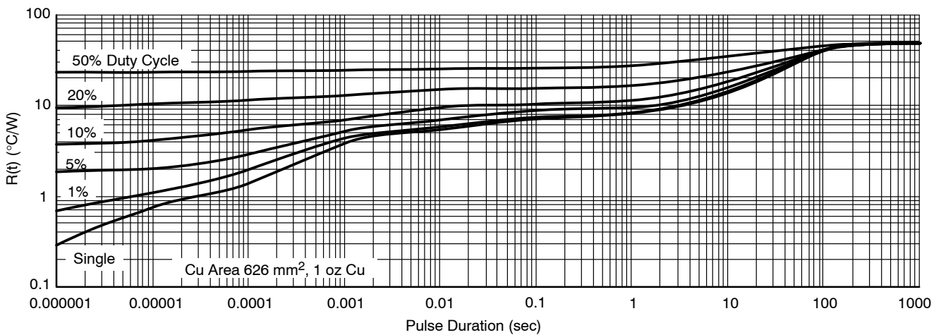
Figure 23. D²PAK 7-Lead Thermal Duty Cycle Curves on 1" Spreader Test Board
