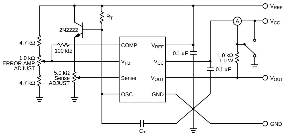
Figure 4. Test Circuit
