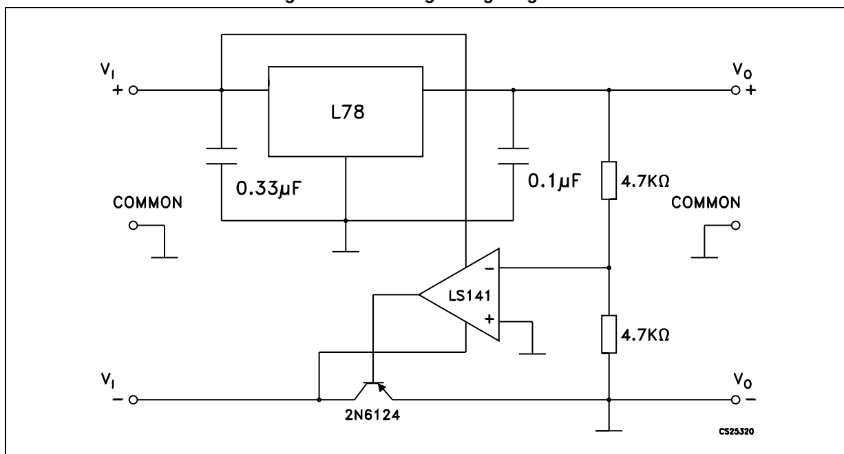
Figure 15. Tracking voltage regulator
