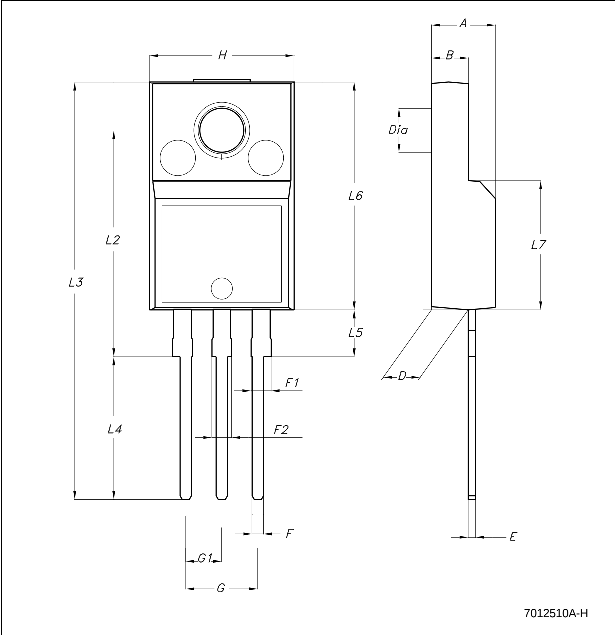
Figure 39. TO-220FP drawing
