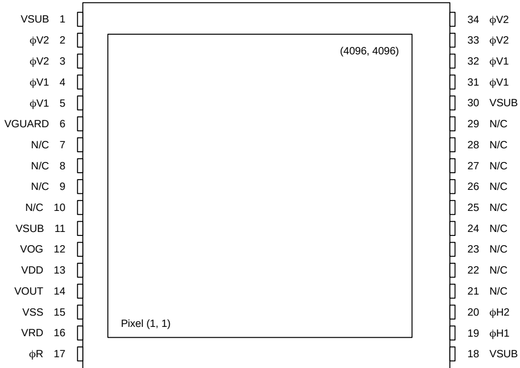
Figure 4. Pinout Diagram
