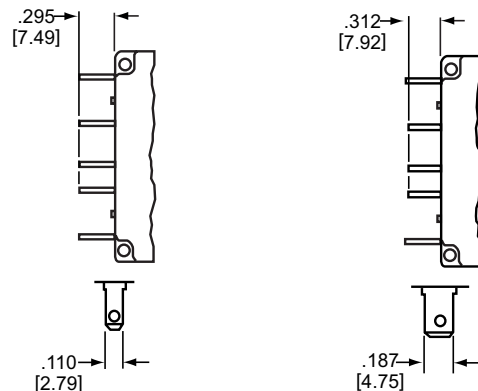
Auxiliary Switch
