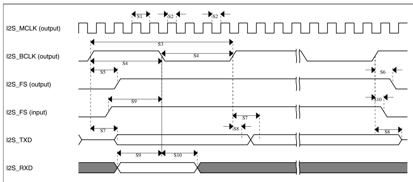
Figure 23. I 2 S timing — master mode
