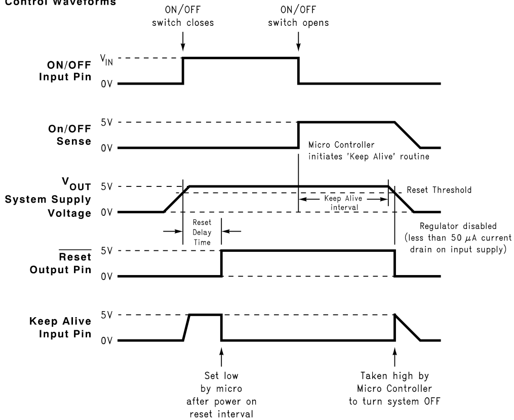
Control Waveforms
