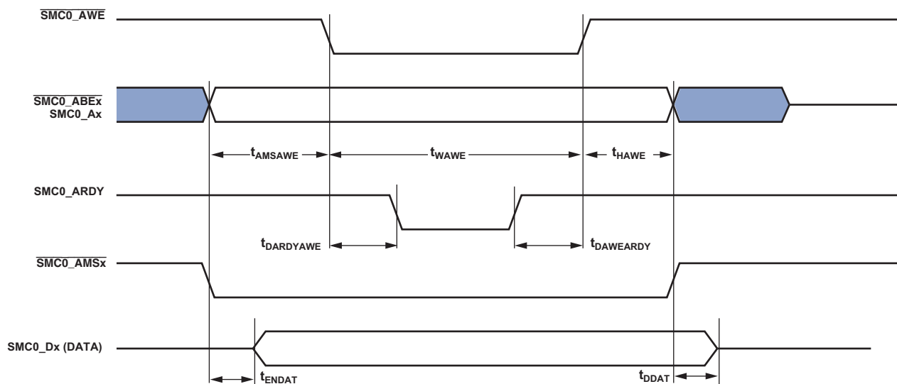
Figure 38. Asynchronous Write
