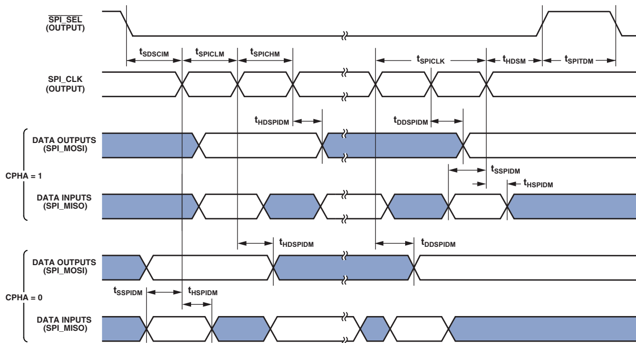
Figure 44. Serial Peripheral Interface (SPI) Port—Master Timing
