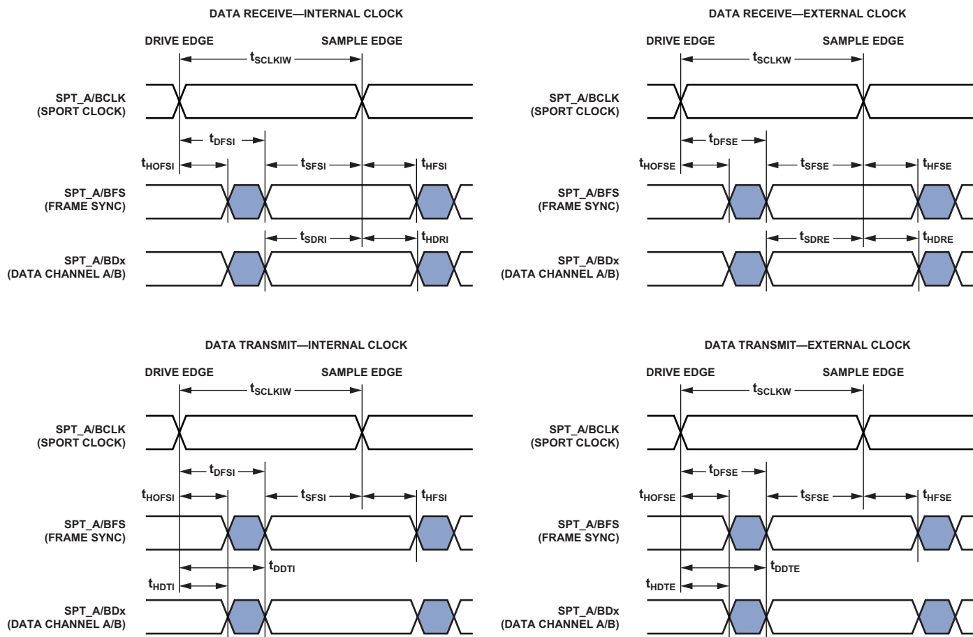
Figure 40. Serial Ports
