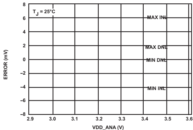
Figure 25. INL Error and DNL Error vs. Supply
