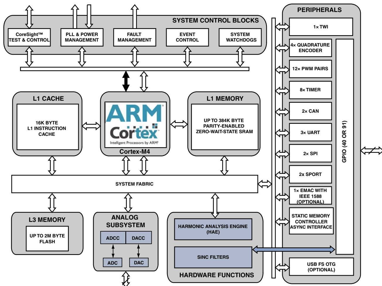
Figure 1. Block Diagram
