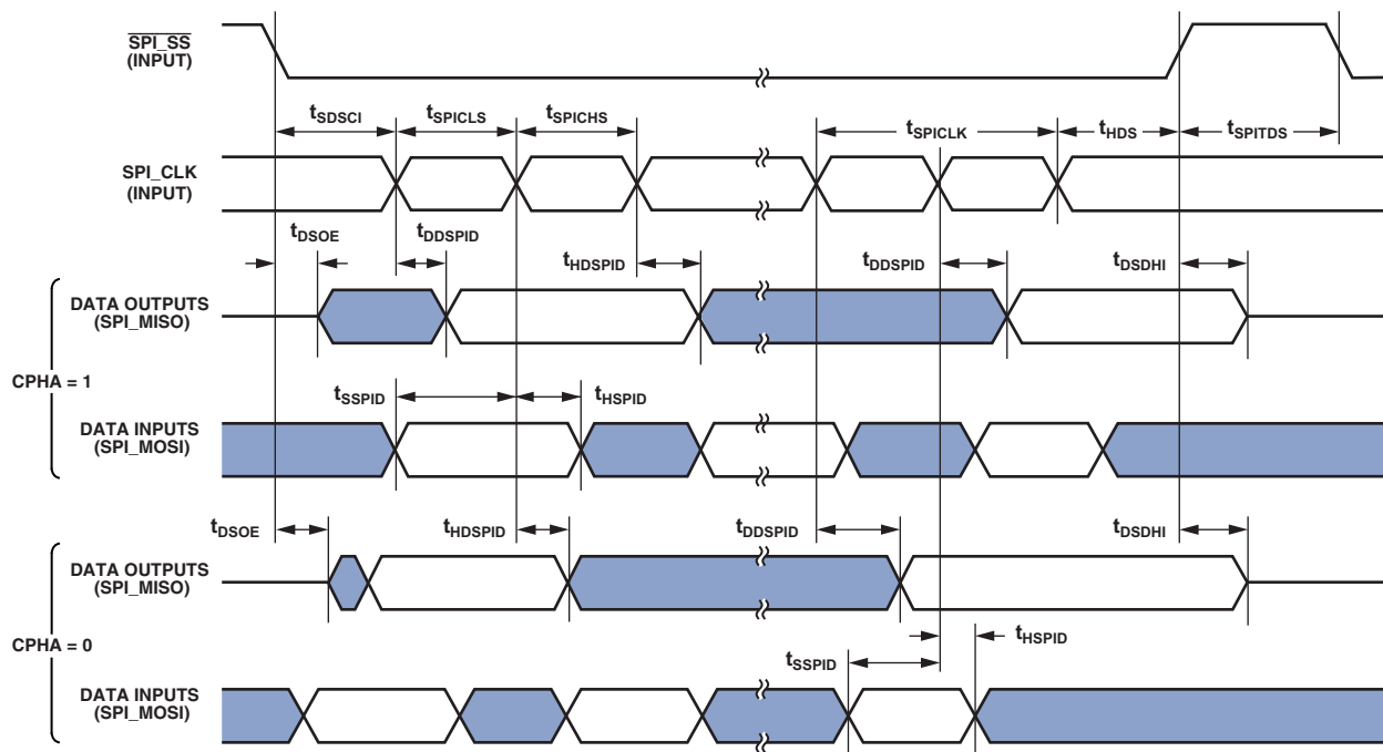
Figure 45. Serial Peripheral Interface (SPI) Port—Slave Timing
