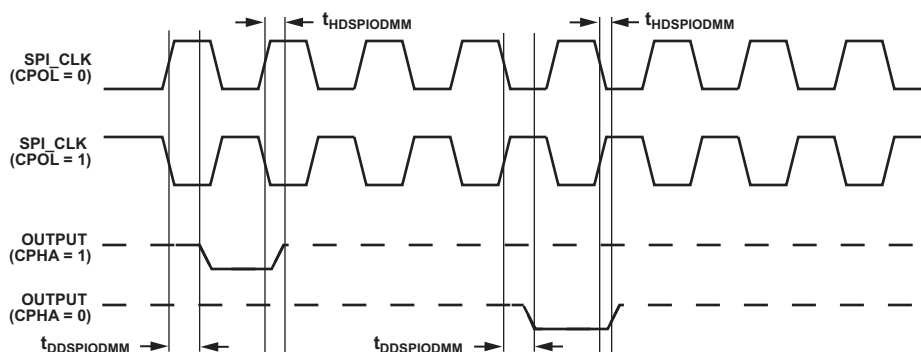
Figure 48. ODM Master
