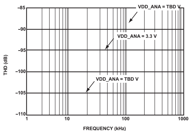
Figure 20. THD vs. Frequency
