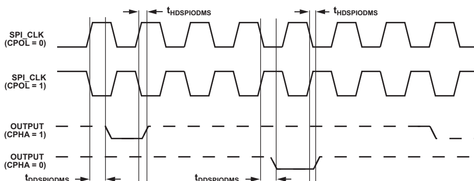
Figure 49. ODM Slave
