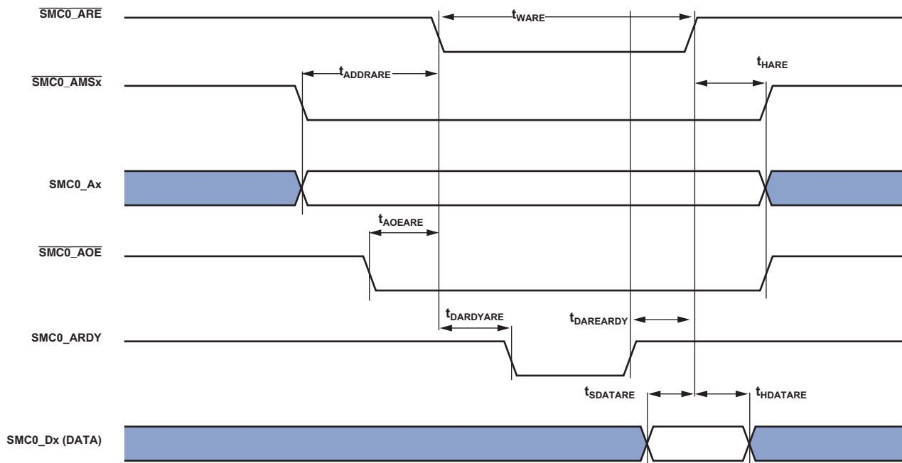
Figure 35. Asynchronous Read
