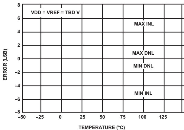
Figure 22. INL Error and DNL Error vs. Temperature
