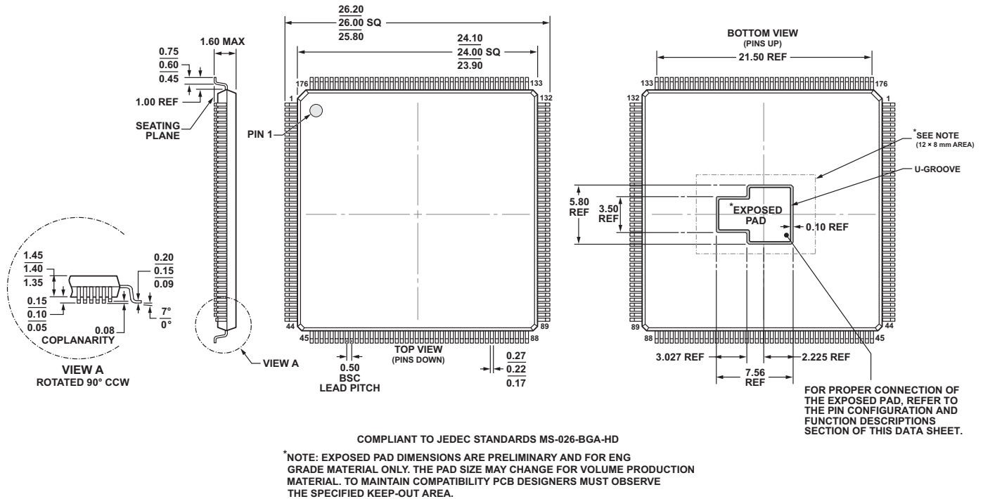
Figure 70. 176-Lead Low Profile Quad Flat Package, Exposed Pad [LQFP_EP] 1 (SW-176-3)
