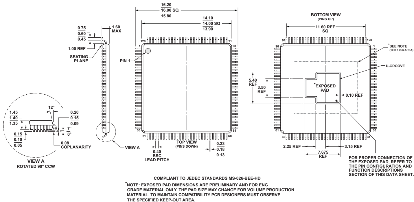
Figure 69. 120-Lead Low Profile Quad Flat Package, Exposed Pad [LQFP_EP] 1 (SW-120-3)
