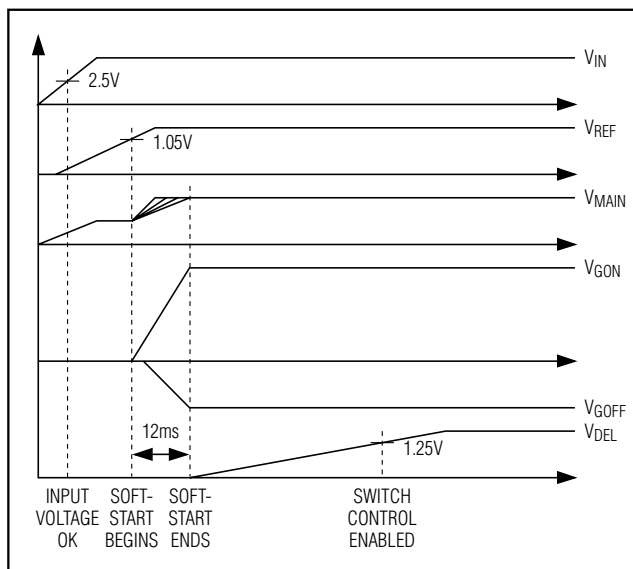
Figure 6. Power-Up Sequence
