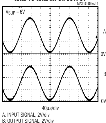
OPERATIONAL-AMPLIFIER RAIL-TO-RAIL INPUT/OUTPUT
