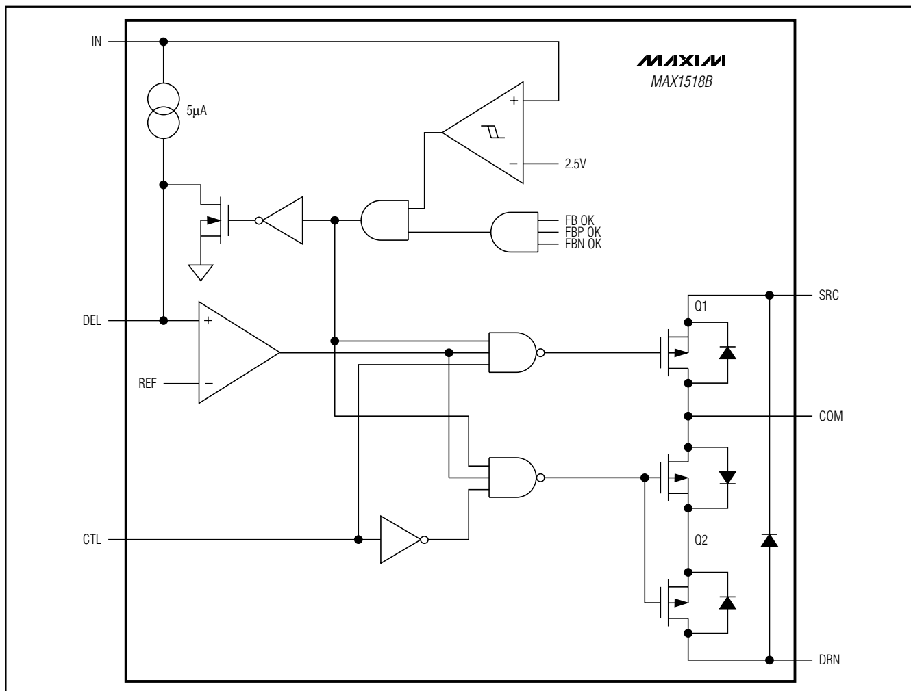
Figure 7. Switch-Control Block
