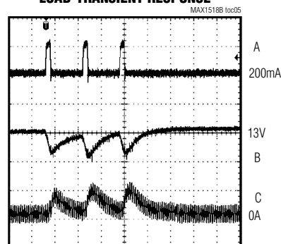
STEP-UP REGULATOR PULSED LOAD-TRANSIENT RESPONSE
