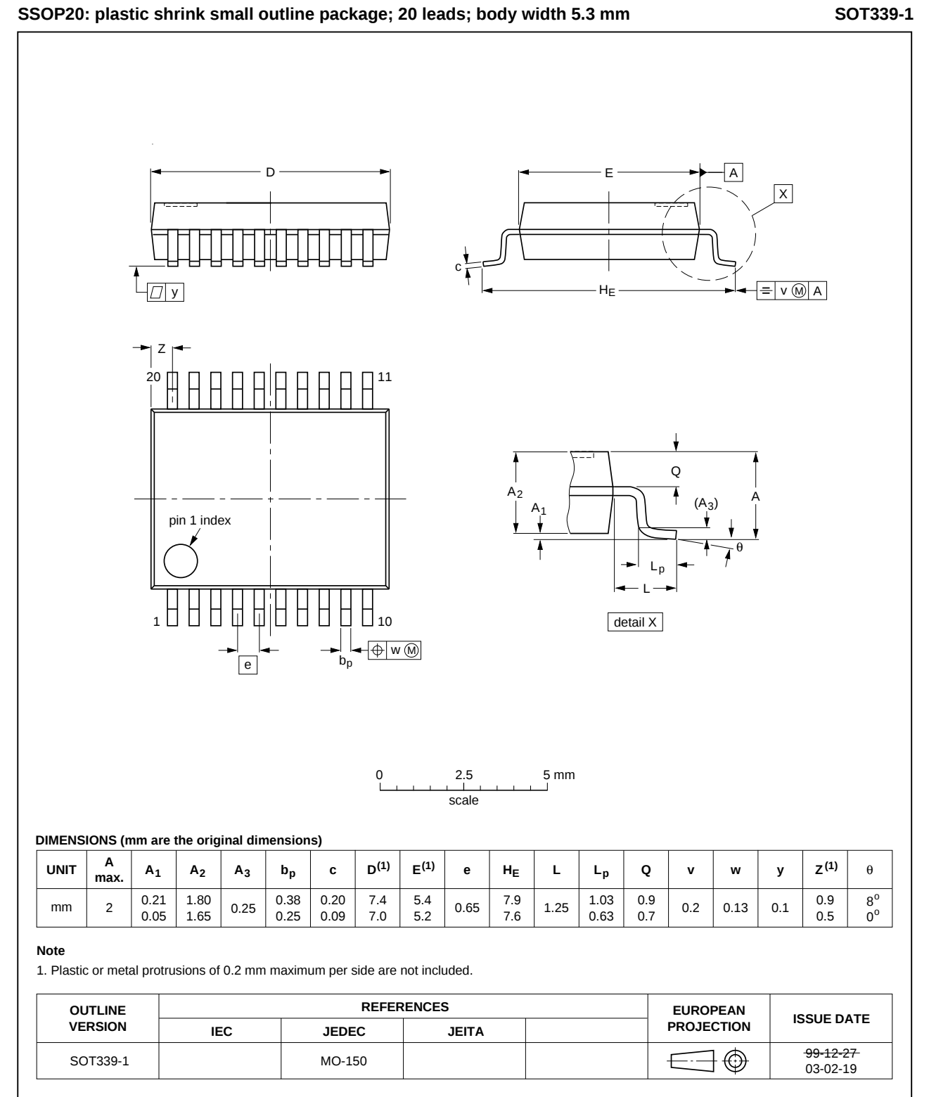
Fig 10. Package outline SOT339-1 (SSOP20)
