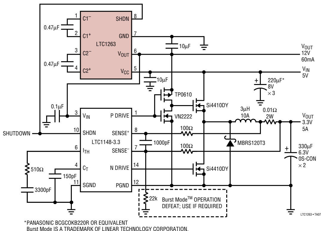
5V to 3.3V/5A Converter with 12V/60mA Auxiliary Output
