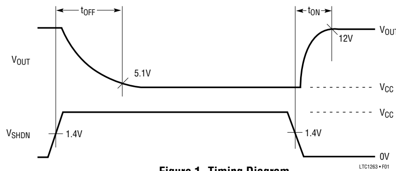
Figure 1. Timing Diagram
