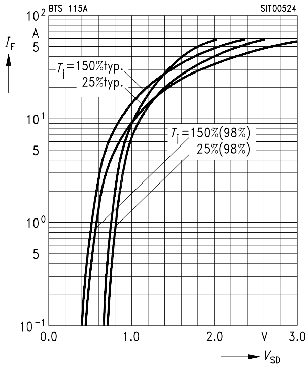
Forward characteristics of reverse diode I_F = f(V_{SD}) Parameter: T_j, t_p = 80 \mu\text{s}
