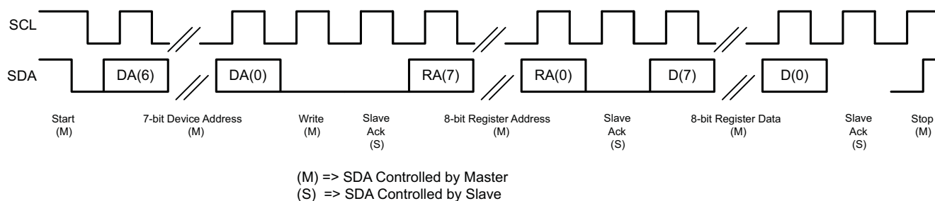
Figure 6-34. I 2 C Write
