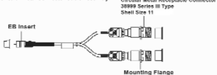
Circular Metal Connector-to-Circular Metal Connector Cable Assembly
