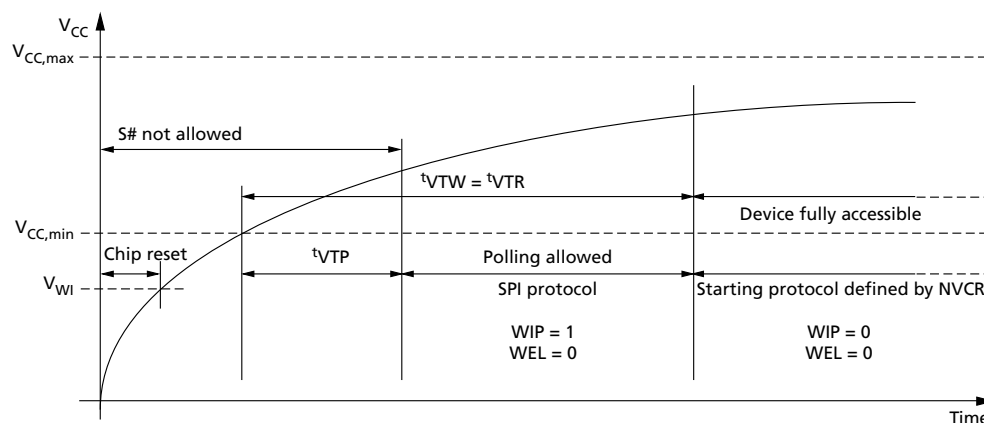
Figure 37: Power-Up Timing
