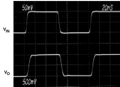
Figure 28. Small Signal Pulse Response, \text{Gain} = +10 , ( R_F = 274 \Omega , R_L = 150 \Omega , V_S = \pm 7.5 \text{ V} )
