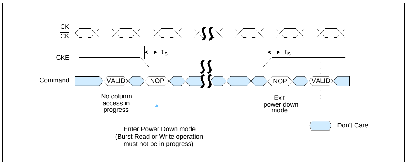
Figure 31 Power Down
