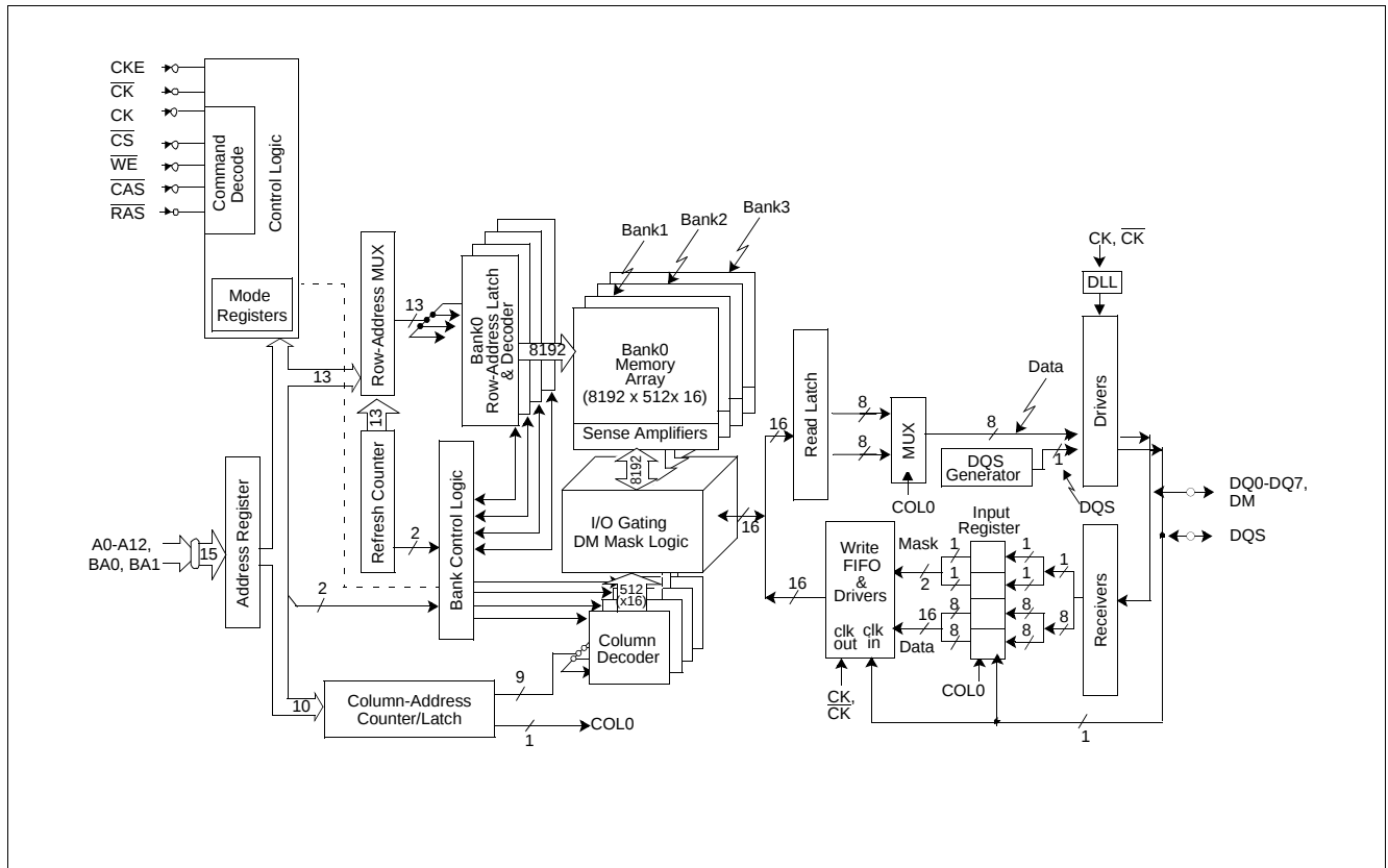
Figure 4 Block Diagram (32Mb × 8)
