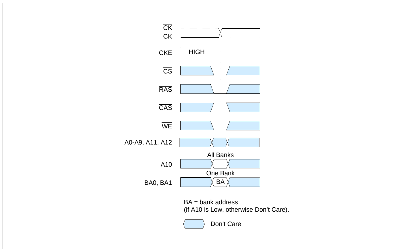
Figure 30 Precharge Command
