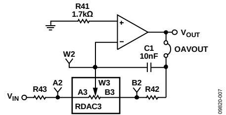
Figure 7. Pseudologarithmic Inverting Amplifier
