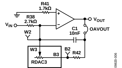
Figure 6. Linear Inverting Amplifier
