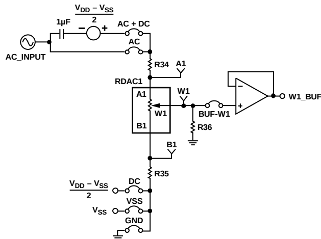
Figure 3. AC Signal Attenuator
