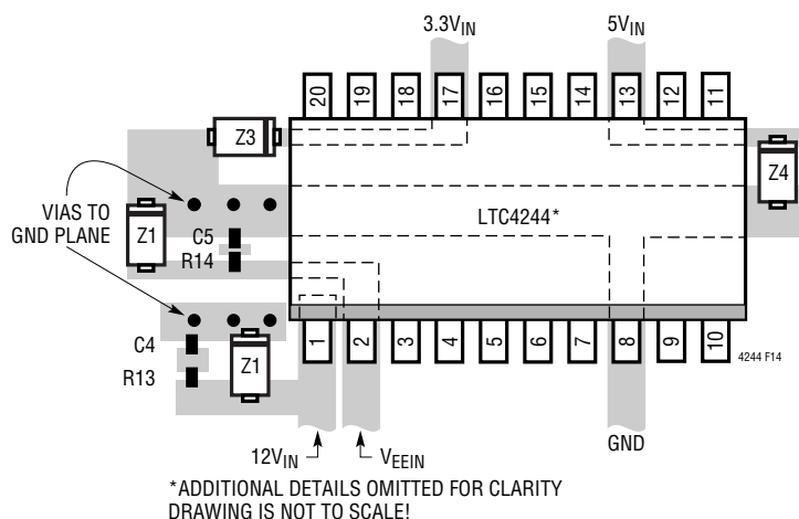
Figure 14. Recommended Layout for Transient Protection Components
