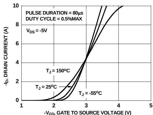
Figure 19. Transfer Characteristics
