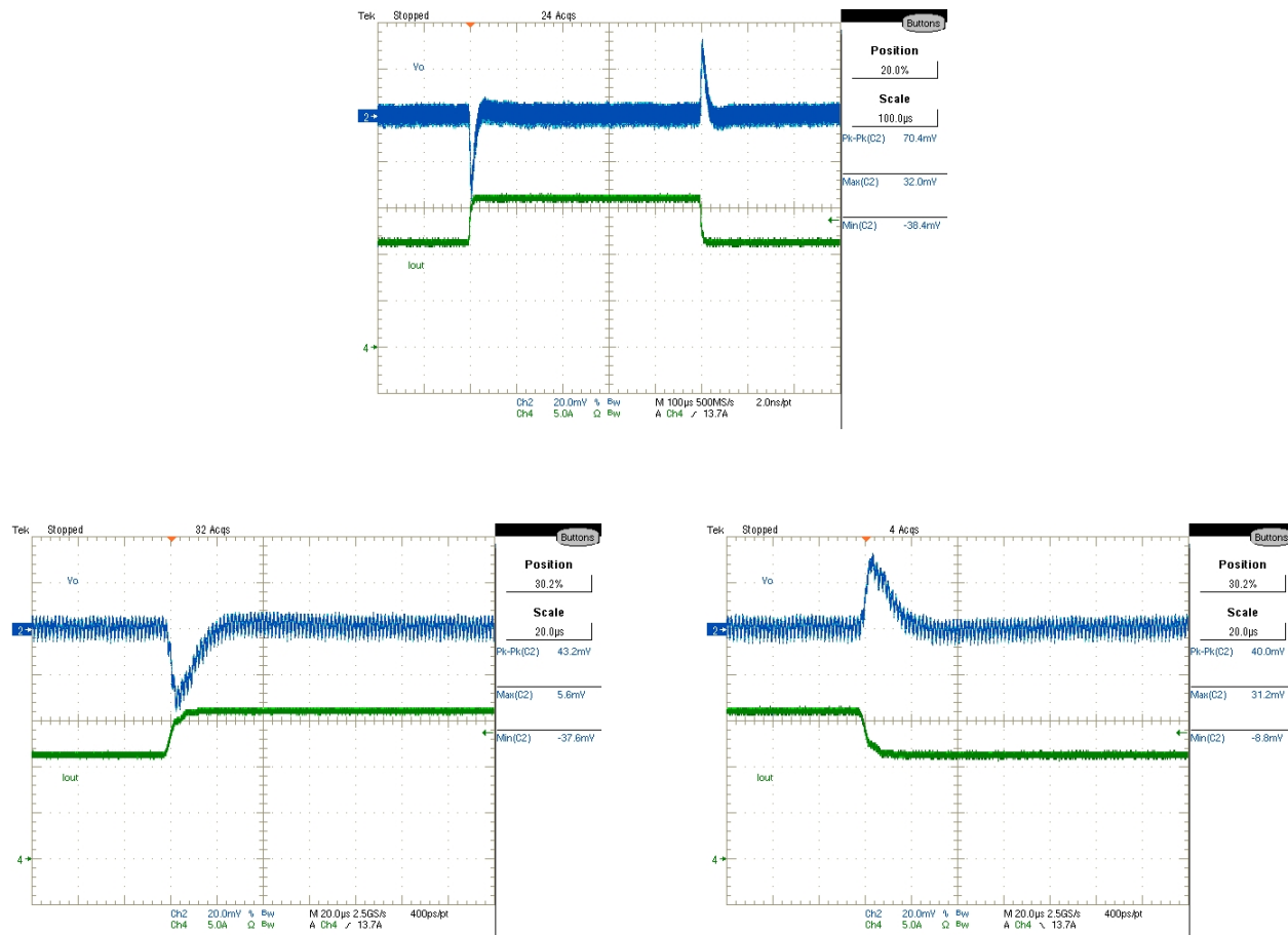
Figure 38: V_{out} Transient Response, 11.2A to 16A step at 2.5A/ \mu Sec CH2: V_{out} , CH4: I_{out}
