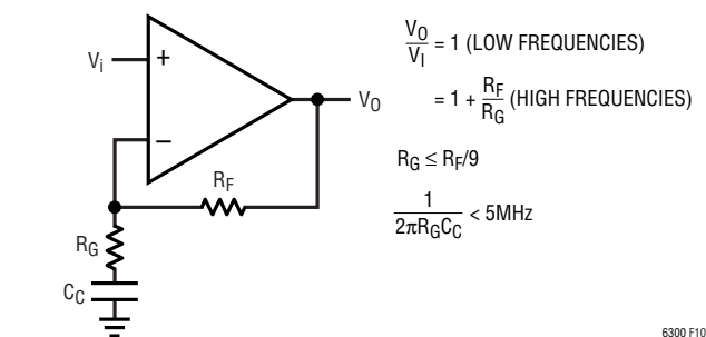
Figure 10. Alternate Noninverting Compensation
