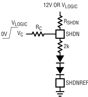
Figure 4. Providing Logic Input Control of Operating Current
