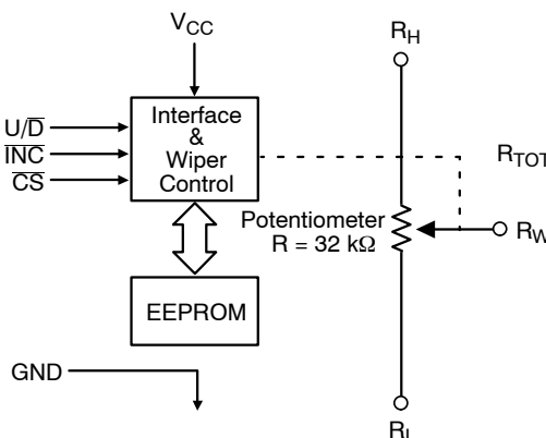
Figure 2. Block Diagram
