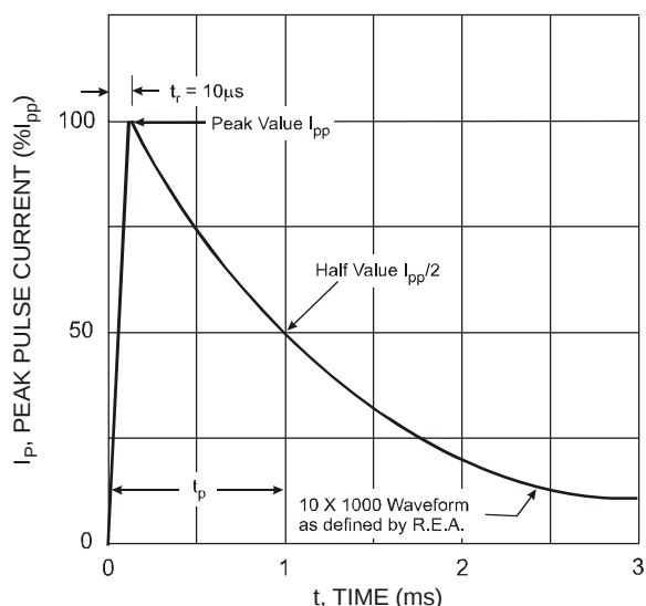
Fig. 4 Pulse Waveform
