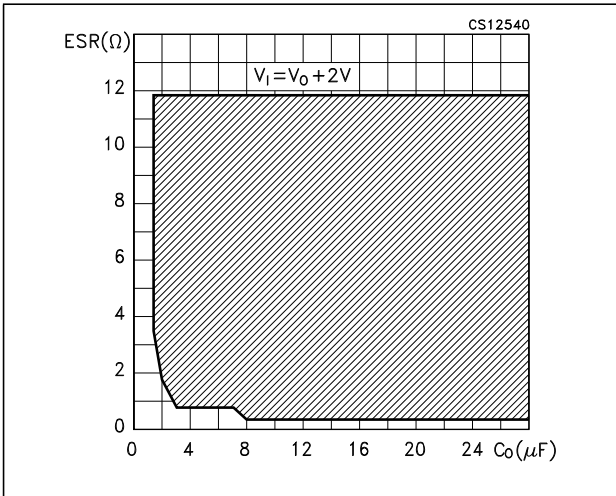
Figure 14. Stability vs. C_O
