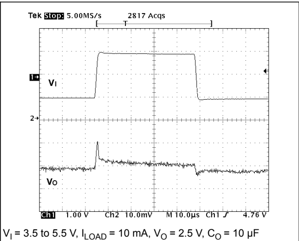
Figure 15. Line transient
