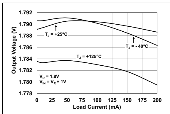
FIGURE 2-9: Output Voltage vs. Load Current ( V_R = 1.8\text{V} ).
