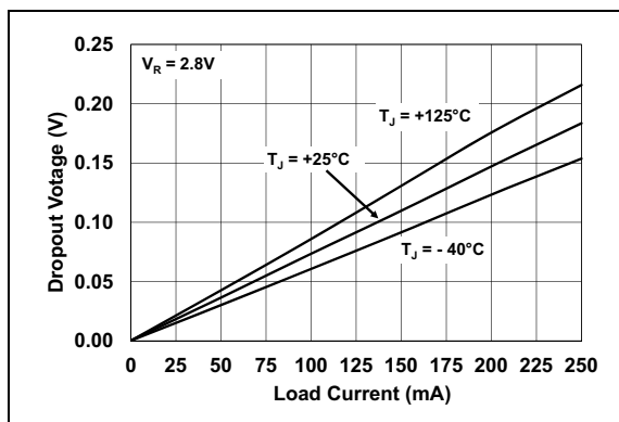
FIGURE 2-12: Dropout Voltage vs. Load Current ( V_R = 2.8\text{V} ).
