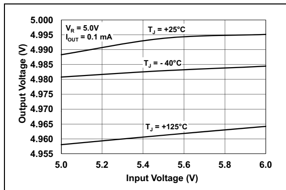
FIGURE 2-7: Output Voltage vs. Input Voltage ( V_R = 5.0\text{V} ).
