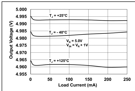
FIGURE 2-11: Output Voltage vs. Load Current ( V_R = 5.0\text{V} ).
