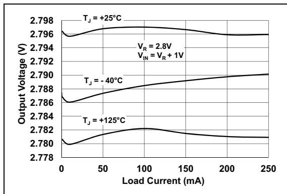
FIGURE 2-10: Output Voltage vs. Load Current ( V_R = 2.8\text{V} ).
