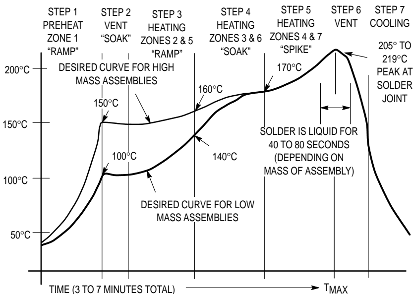
Figure 23. Typical Solder Heating Profile
