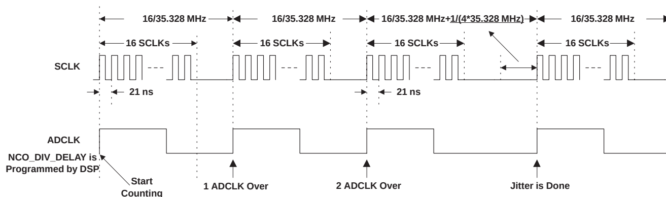
Figure 8. ADCLK Jitter Example
