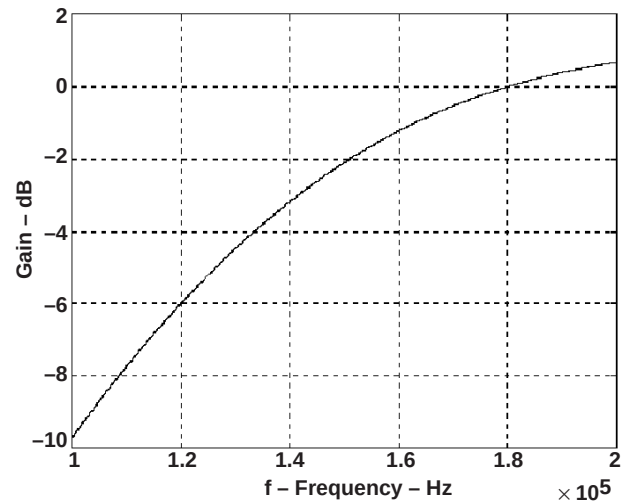
(b) RX-Stage HPF1 Frequency Response (100 kHz to 200 kHz)
