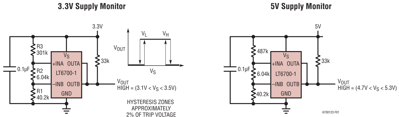
Figure 1. Simple Window Comparator
