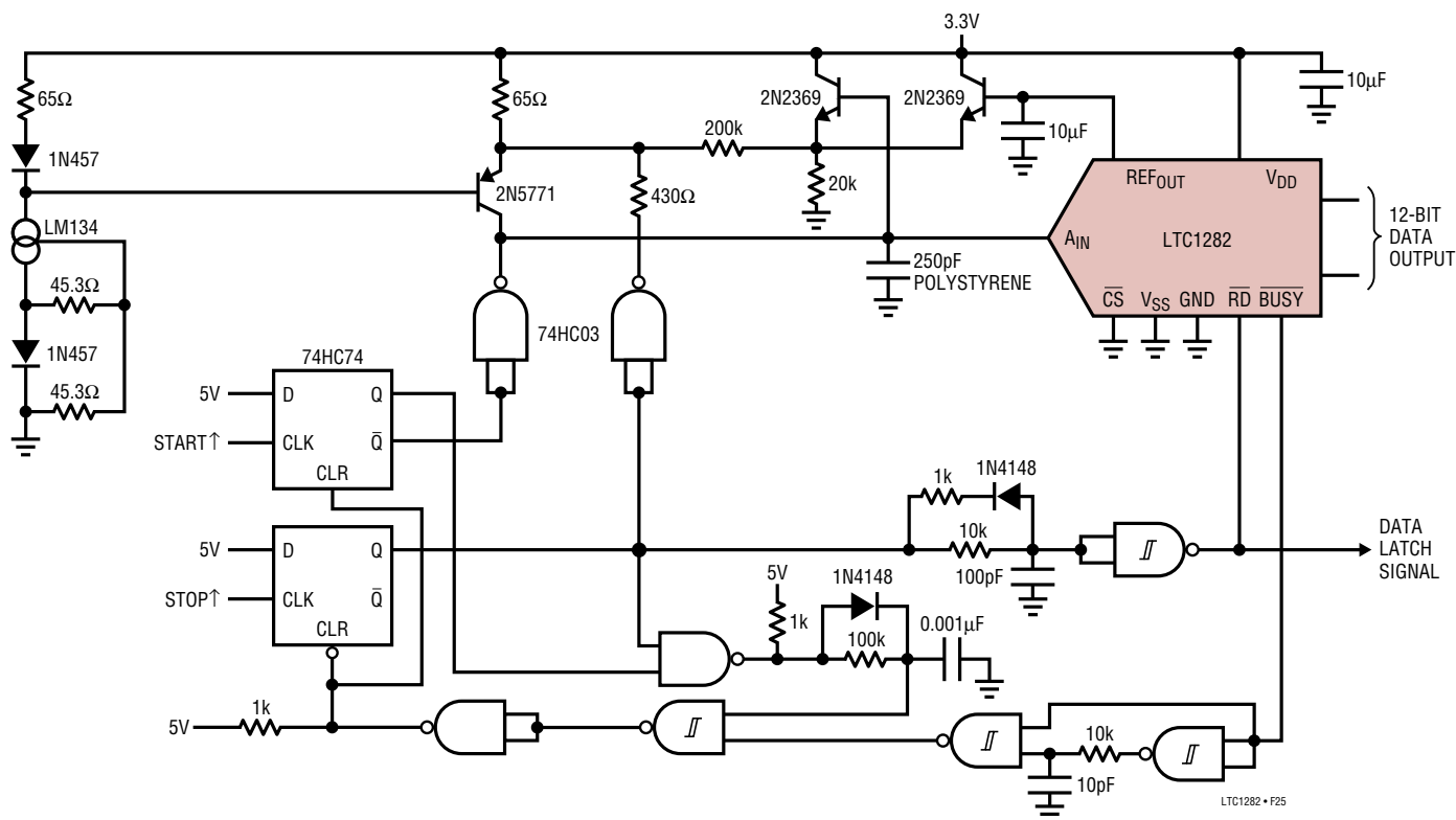
Figure 25. \Delta Time Measurement with the LTC1282
