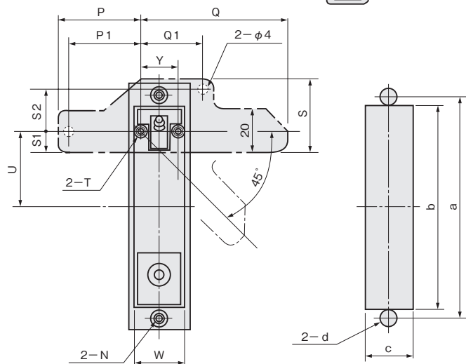
Layout of Holes for Installation
