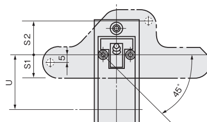
Shape of cam for THA-203-4-THA-190-3
