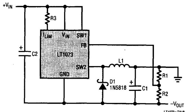
Figure 8. Positive-to-Negative Converter
