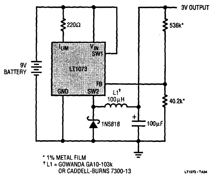
9V to 3V Step-Down Converter
