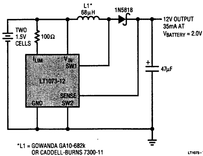
3V to 12V Step-Up Converter
