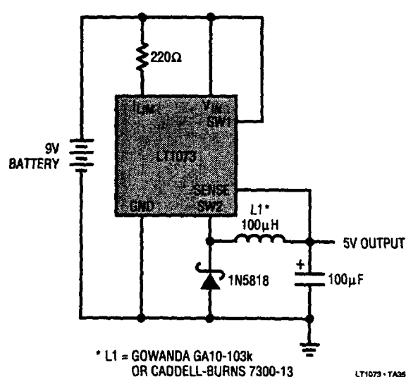
9V to 5V Step-Down Converter
