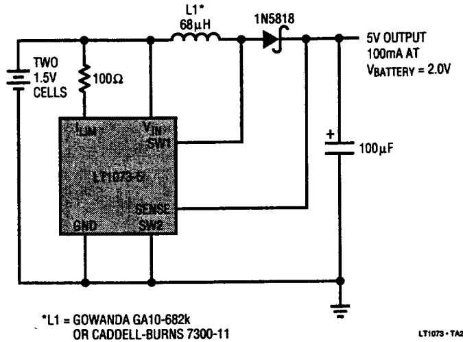
3V to 5V Step-Up Converter
