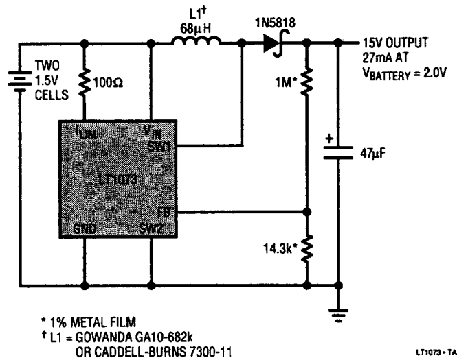
3V to 15V Step-Up Converter
