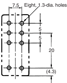
Mounting Holes
