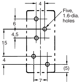
Mounting Holes
