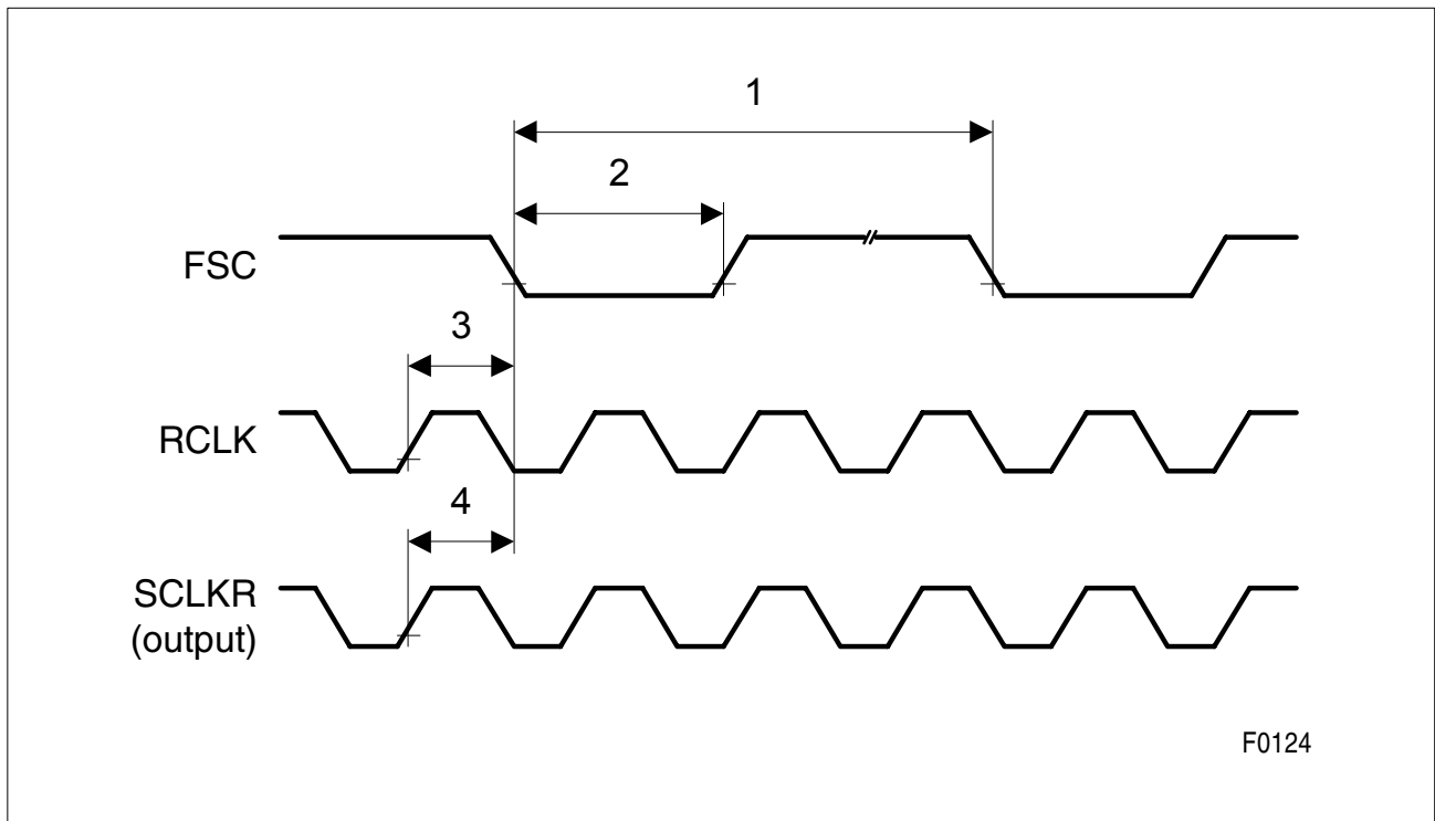
Figure 101 FSC Timing
