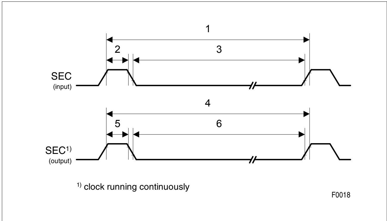
Figure 100 SEC Timing
