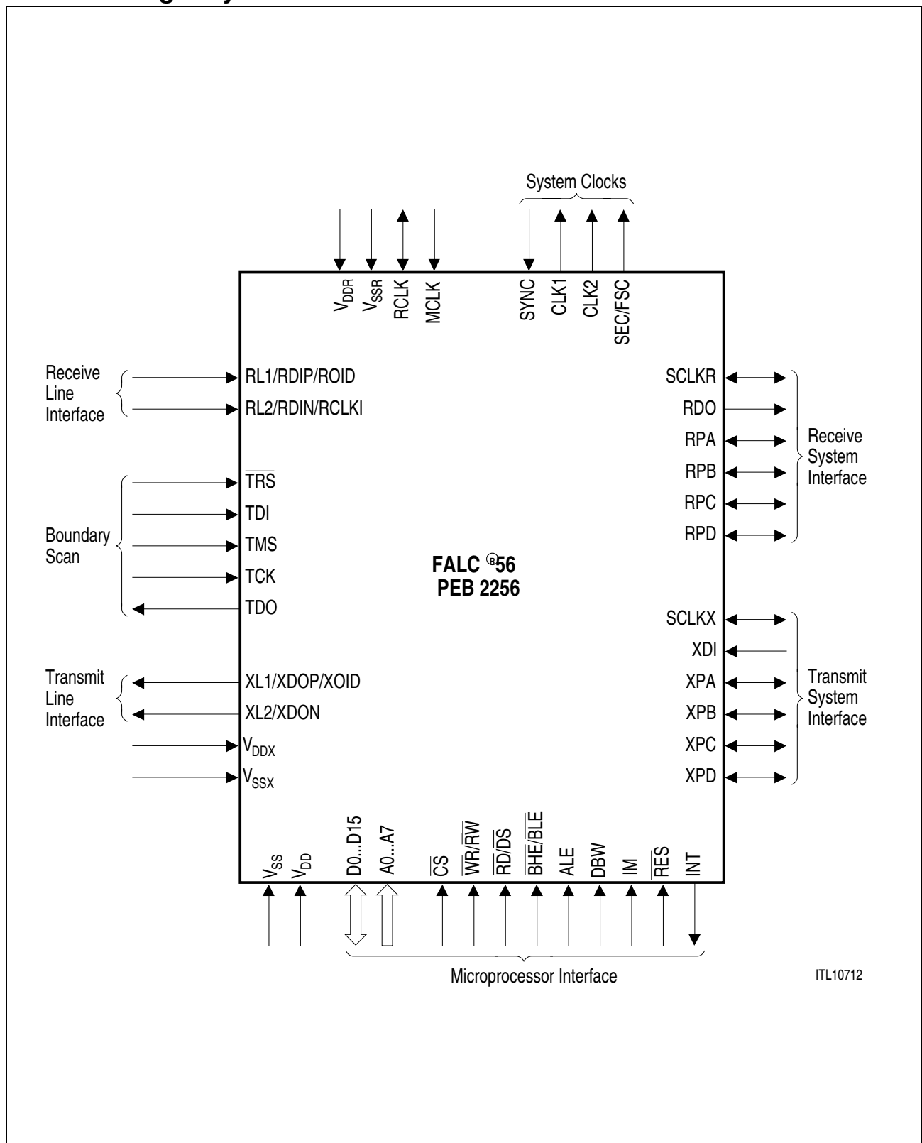
Figure 1 Logic Symbol
