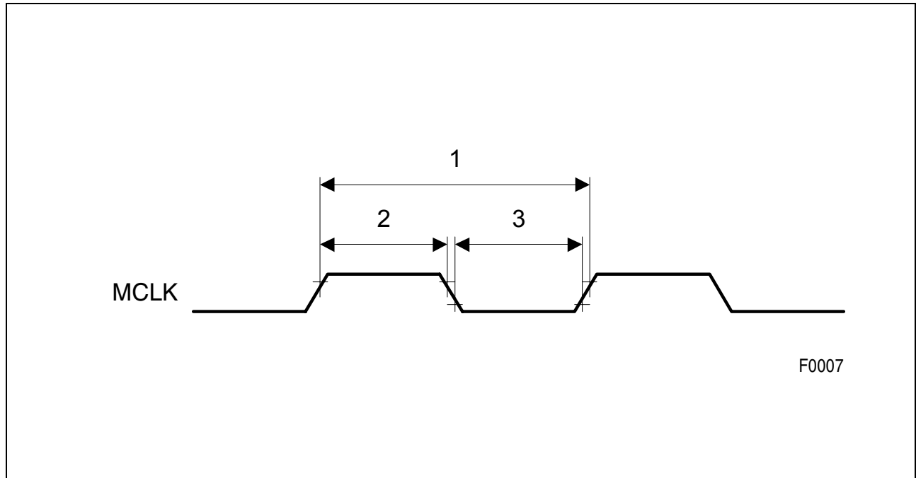
Figure 81 MCLK Timing
