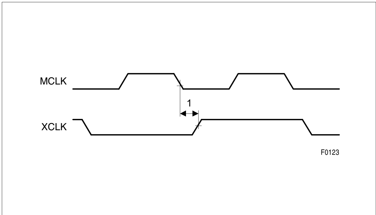
Figure 99 XCLK Timing
