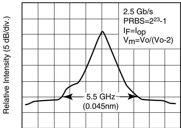
Fig. 1 Lasing Spectrum
