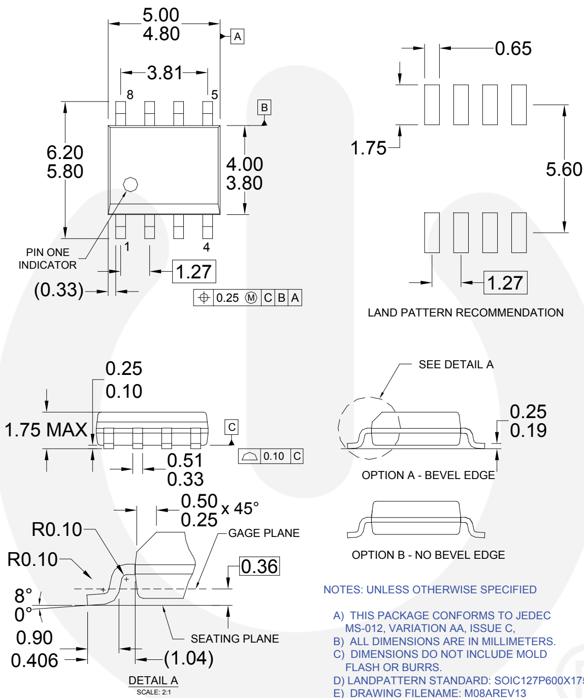
Figure 18. SOIC-8 Package
