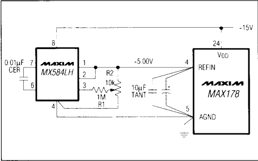
Figure 18. MX584LH as Reference Generator
