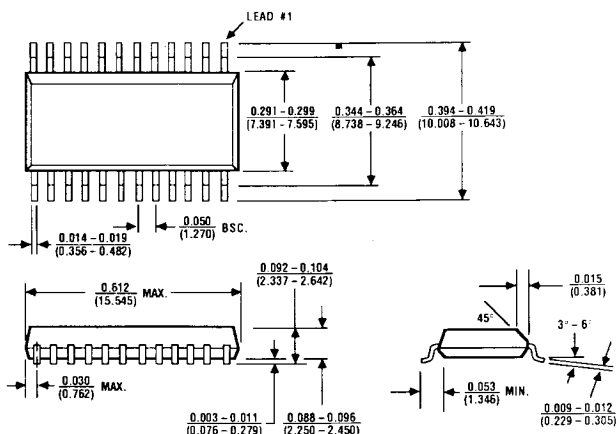
24 Lead Small Outline, Wide (WG)
