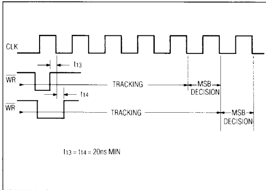
Figure 7. Width of Tracking Interval as a Function of WR Rising Edge Timing with Respect to CLK Falling Edge
