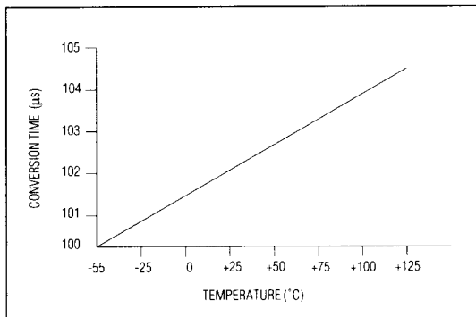
Figure 10. Typical Change in Conversion Time Variation vs. Temperature when Using Internal Clock
