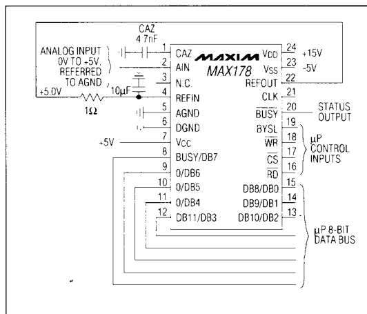
Figure 5. MAX178 Operational Diagram
