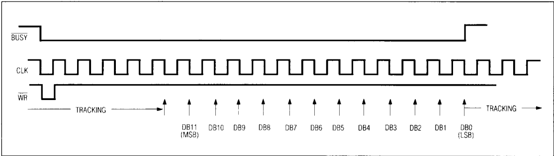
Figure 6. MAX178 Timing Diagram
