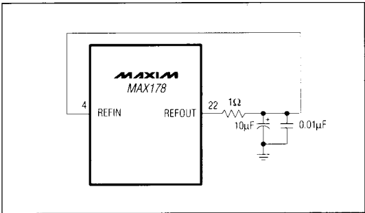
Figure 16. Internal Reference Hookup. Note: Reference Value Is Not Adjustable.
