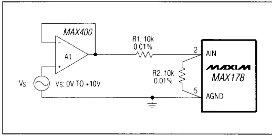
Figure 13. Unipolar 0V to +10V Operation
