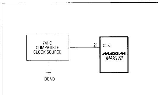
Figure 9. External Clock Operation
