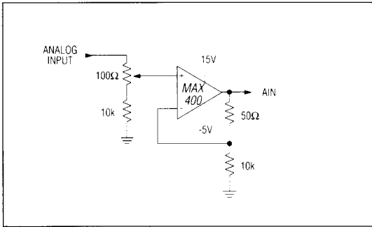
Figure 17. Adjusting Analog Input Gain to Trim Out Initial Reference Voltage Error
