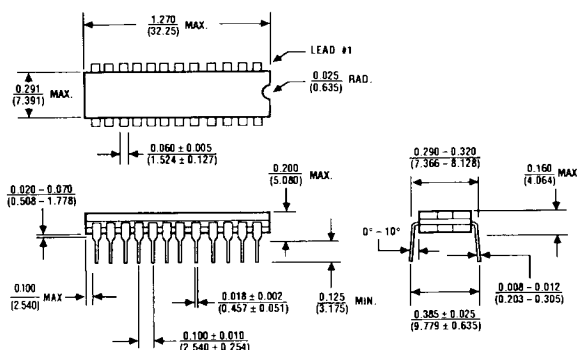
24 Lead Narrow Cerdip (RG)
