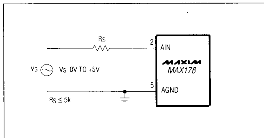
Figure 11. Unipolar 0V to +5V Operation
