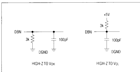
Figure 3. Load Circuits for Access Time Test ( t_{11} )
