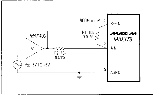
Figure 14. Bipolar -5V to +5V Operation
