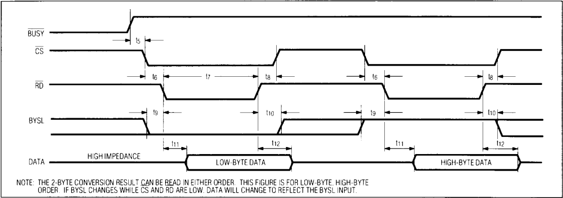
Figure 2. Read Cycle Timing
