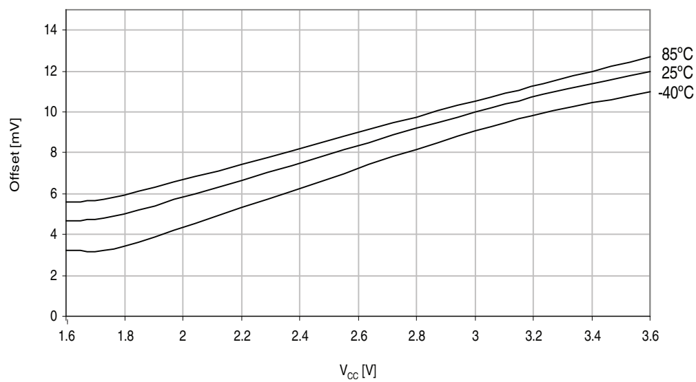
Figure 37-28. ADC Offset vs. V_{CC} . SE Unsigned mode, V_{REF} = 1.0V , external reference.
