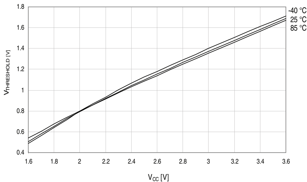
Figure 37-56. Reset pin input threshold voltage vs. V_{CC} .
