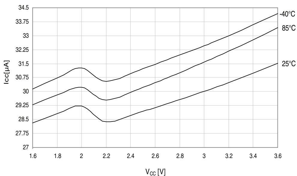
Figure 37-8. Idle mode supply current vs. V_{CC} .
