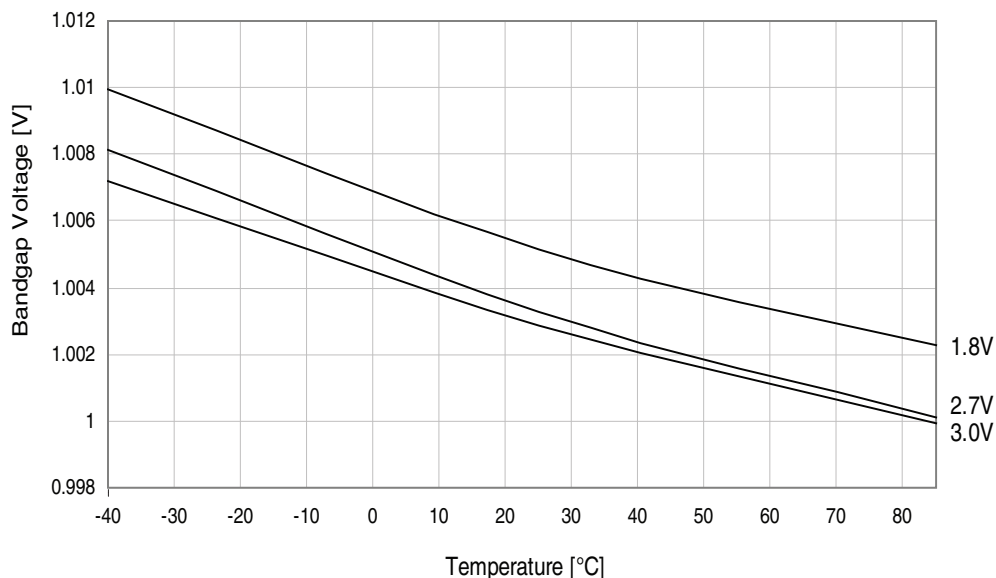
Figure 37-45. ADC/DAC Internal 1.0V reference vs. temperature.
