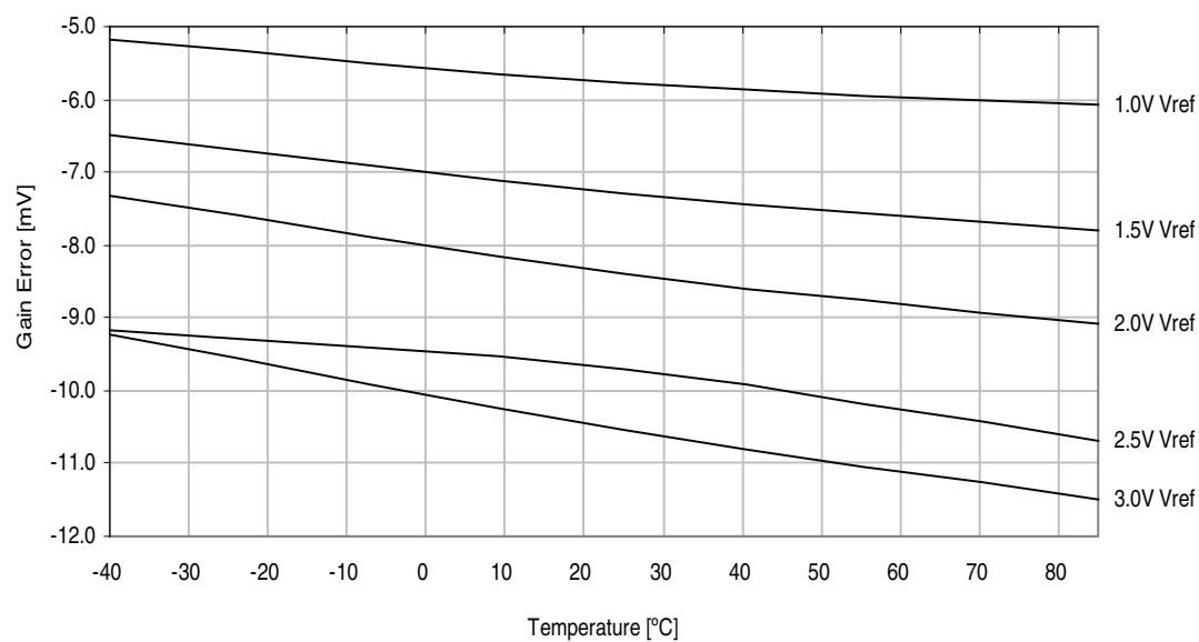
Figure 37-36. ADC Gain Error vs. Temperature. Differential signed mode, external reference.
