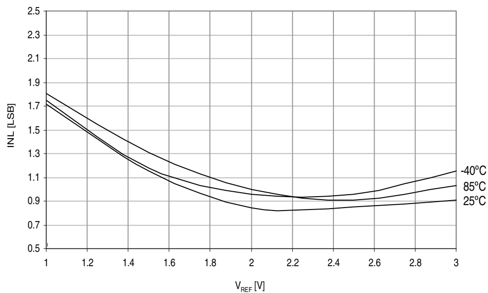
Figure 37-24. ADC INL vs. V_{REF} .
