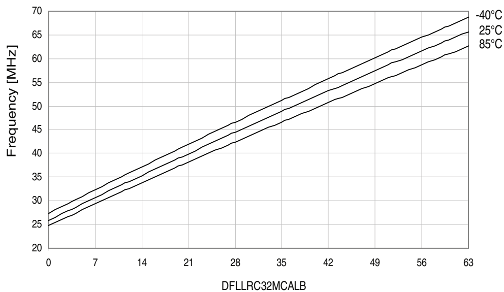
Figure 37-70. 32MHz internal oscillator frequency vs. CALB calibration value.
