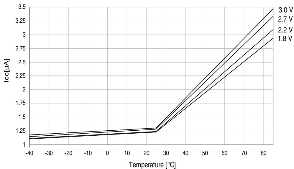
Figure 37-11. Power-down mode supply current vs. Temperature. Watchdog and sampled BOD enabled.
