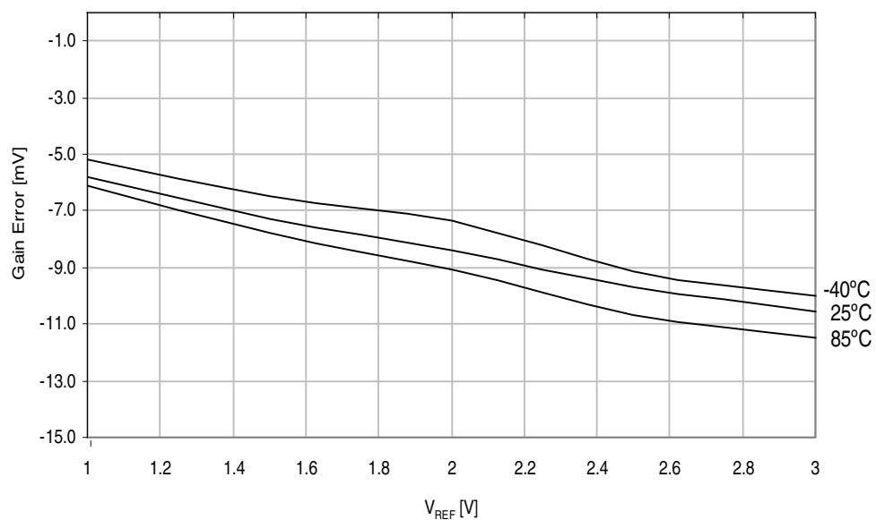
Figure 37-32. ADC Gain Error vs. V_{REF} . Differential signed mode, external reference.
