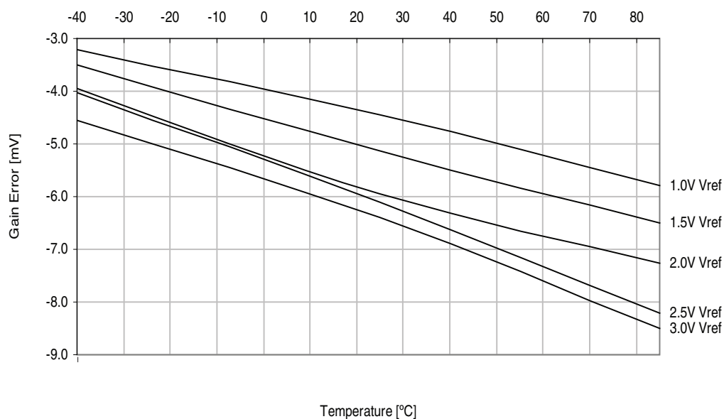
Figure 37-37. ADC Gain Error vs. Temperature. SE Unsigned mode, V_{CC} = 3.6V , external reference.
