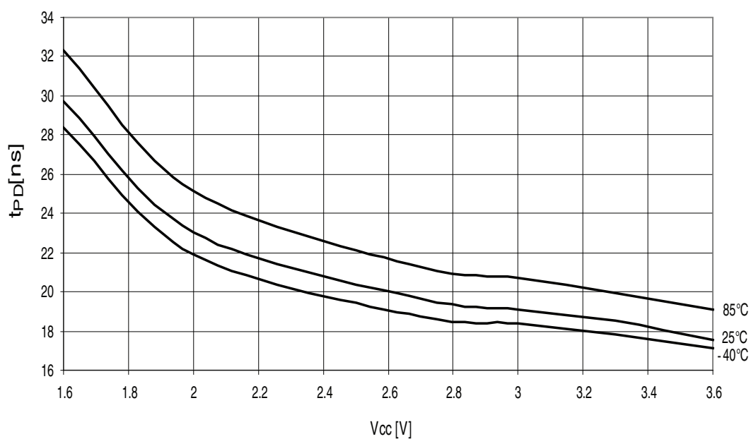
Figure 37-40. Analog comparator propagation delay vs. V_{CC} . High speed mode.
