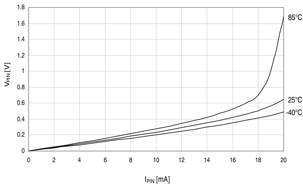
Figure 37-18. I/O pin output voltage vs. sink current.
