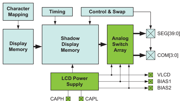
Figure 28-1. LCD overview
