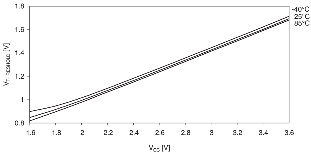
Figure 37-21. I/O pin input threshold voltage vs. V_{CC} . V_{IH} I/O pin read as "1".
