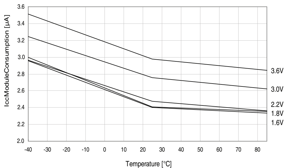
Figure 37-82. Psave LCD LP 32Hz vs. Temperature RTC, WDT, BOD sampled
