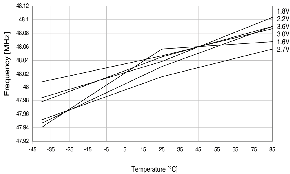
Figure 37-72. 48MHz internal oscillator frequency vs. temperature. DFLL enabled, from the 32.768kHz internal oscillator.
