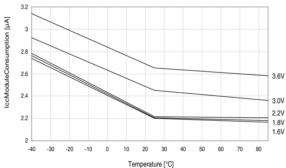
Figure 37-81. Psave LCD LP 32Hz vs. Temperature
