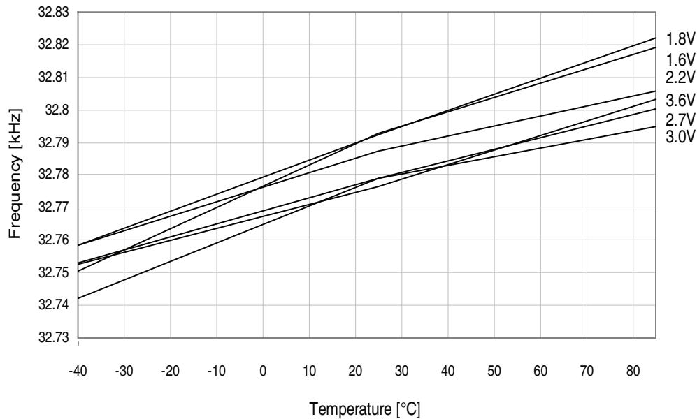
Figure 37-58. 32.768kHz ULP internal oscillator frequency vs. temperature.
