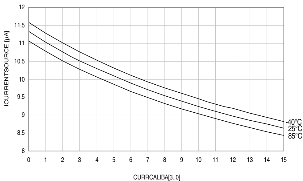
Figure 37-44. Analog comparator current source vs. Calibration. V CC = 3.0V, double mode.
