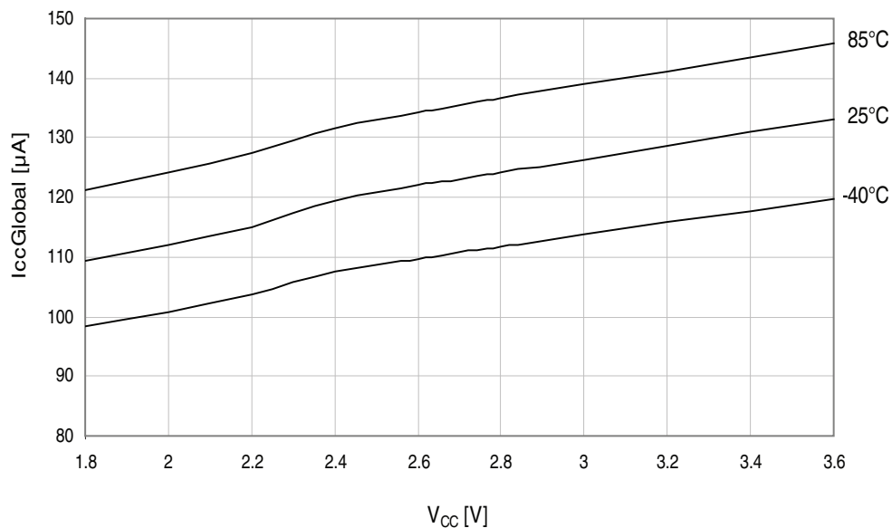
Figure 37-46. BOD current consumption vs. V_{CC} . Continuous mode, BOD level = 1.6V.
