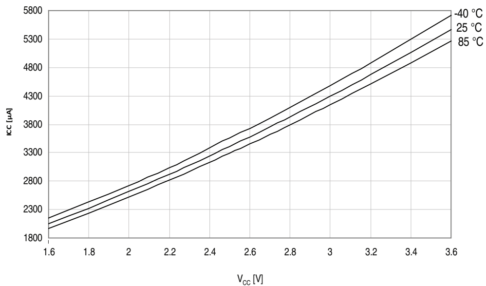
Figure 37-9. Idle mode current vs. V_{CC} . f_{SYS} = 32\text{MHz} internal oscillator.
