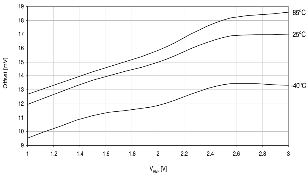
Figure 37-29. ADC Offset vs. V_{REF} SE Unsigned mode, V_{CC} = 3.6V , external reference.
