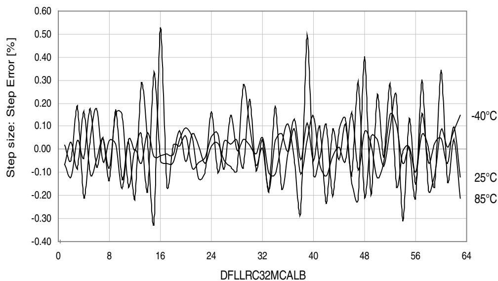
Figure 37-68. 32MHz internal oscillator CALB calibration step size.
