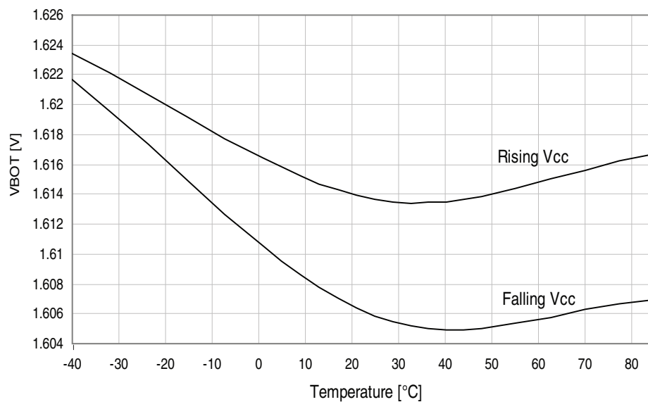
Figure 37-48. BOD thresholds vs. temperature. BOD level = 1.6V.
