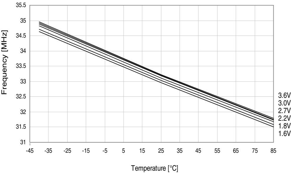
Figure 37-66. 32MHz internal oscillator frequency vs. temperature. DFLL enabled, from the 32.768kHz internal oscillator.
