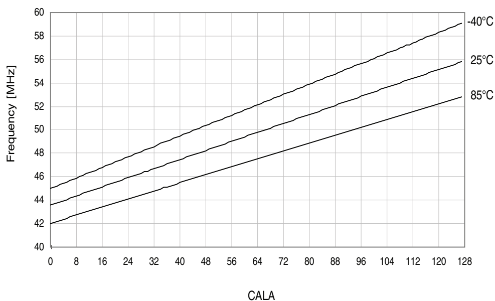
Figure 37-74. 48MHz internal oscillator frequency vs. CALA calibration value. V_{CC} = 3.0V .
