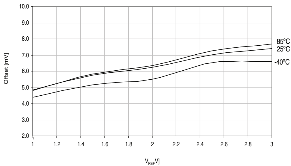
Figure 37-30. ADC Offset vs. V_{REF} Differential signed mode, V_{CC} = 3.6V , external reference.
