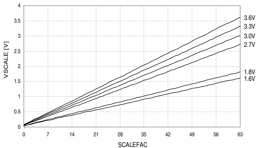
Figure 37-42. Analog comparator voltage scaler vs. SCALEFAC. T = 25^\circ C .
