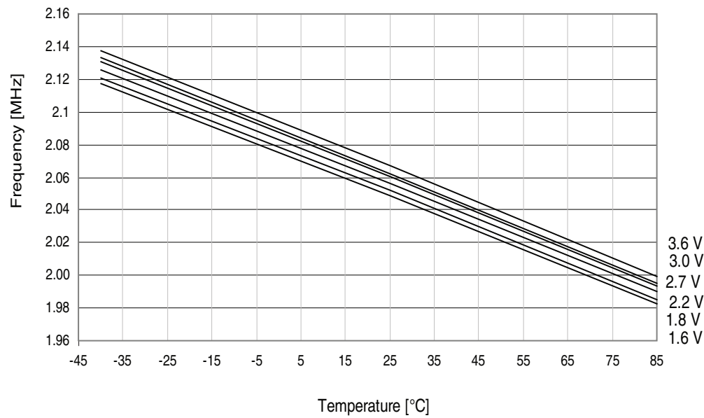
Figure 37-61. 2MHz internal oscillator frequency vs. temperature. DFLL disabled.
