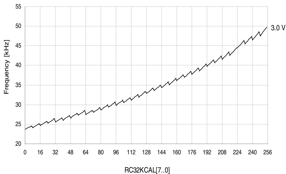
Figure 37-60. 32.768kHz internal oscillator frequency vs. calibration value.
