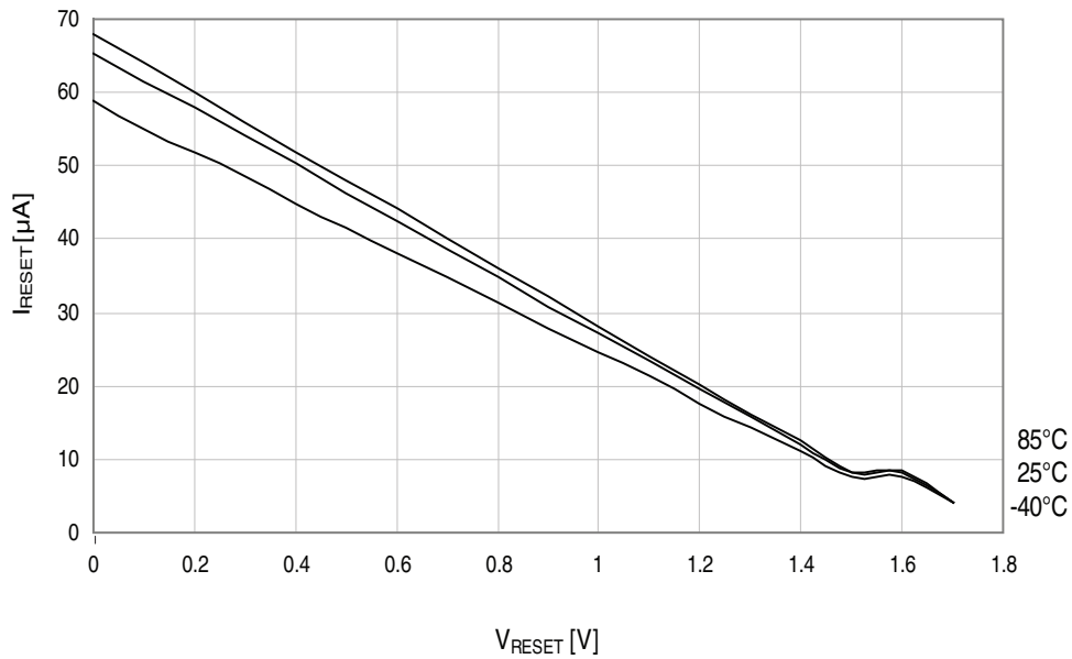
Figure 37-52. Reset pin pull-up resistor current vs. reset pin voltage.
