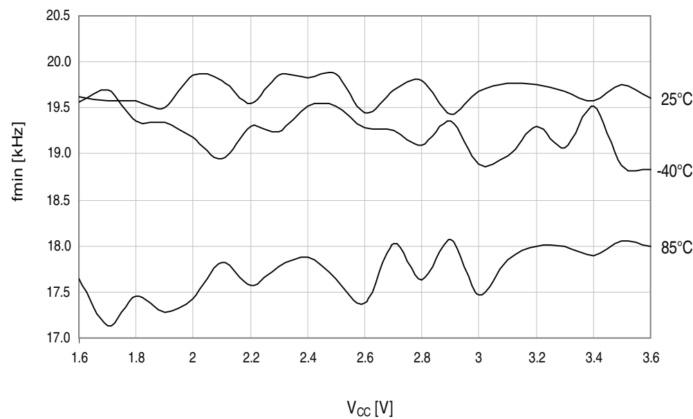
Figure 37-75. Maximum PDI frequency vs. V_{CC} .
