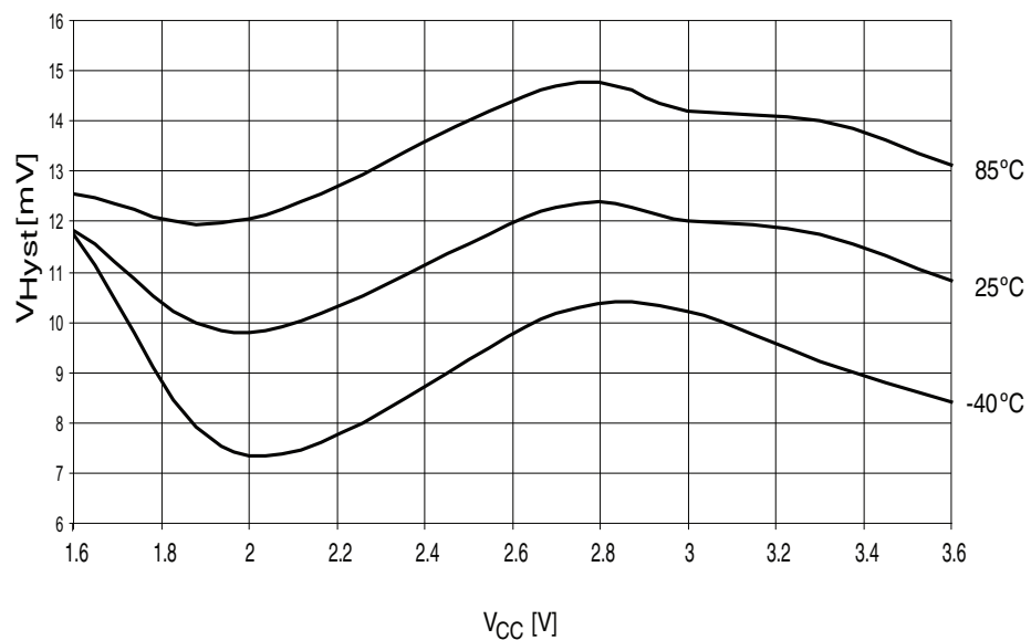
Figure 37-38. Analog comparator hysteresis vs. V_{CC} . High-speed mode, small hysteresis.
