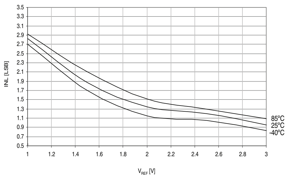
Figure 37-25. ADC INL vs. V_{REF} . SE Unsigned mode, V_{CC} = 3.6V , external reference.
