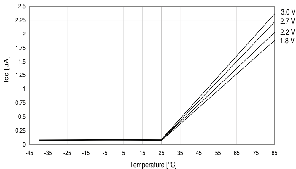
Figure 37-10. Power-down mode supply current vs. Temperature. All functions disabled.
