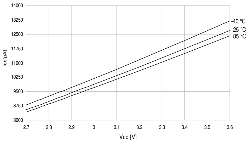
Figure 37-4. Active mode supply current vs. V_{CC} .
