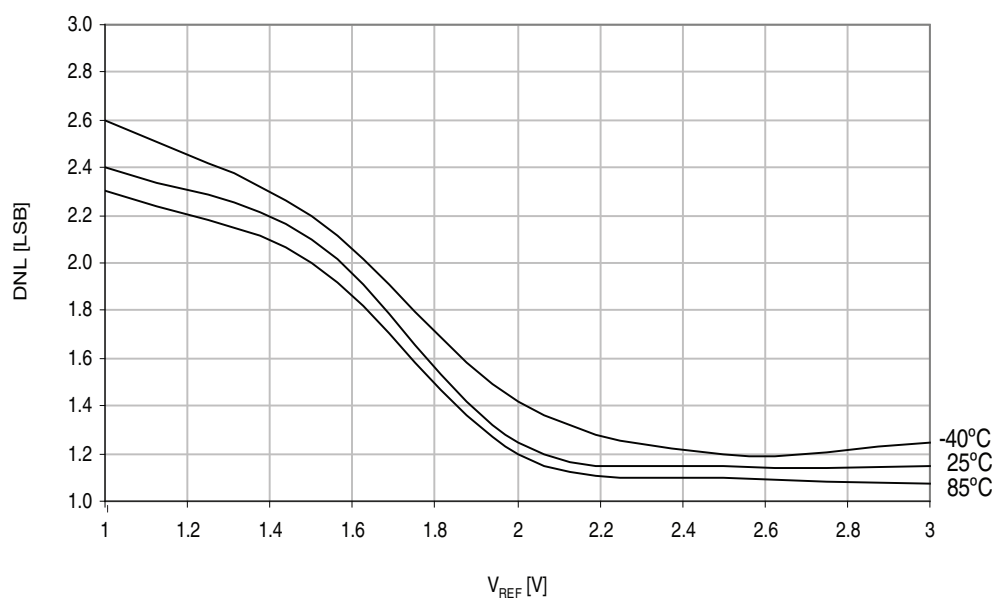
Figure 37-27. ADC DNL vs. V_{REF} . SE Unsigned mode, V_{CC} = 3.6V , external reference.
