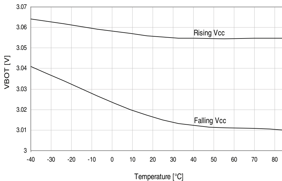
Figure 37-50. BOD thresholds vs. temperature.
