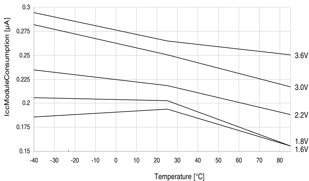
Figure 37-83. Psave vs. Temperature RTC, WDT, BOD sampled.
