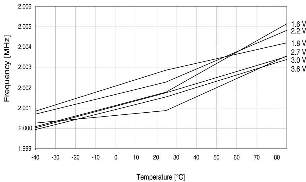
Figure 37-62. 2MHz internal oscillator frequency vs. temperature. DFLL enabled.
