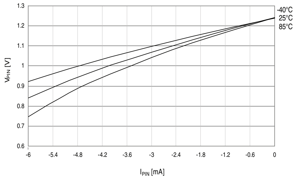
Figure 37-16. I/O pin output voltage vs. source current. V_{CC} = 3.0V .
