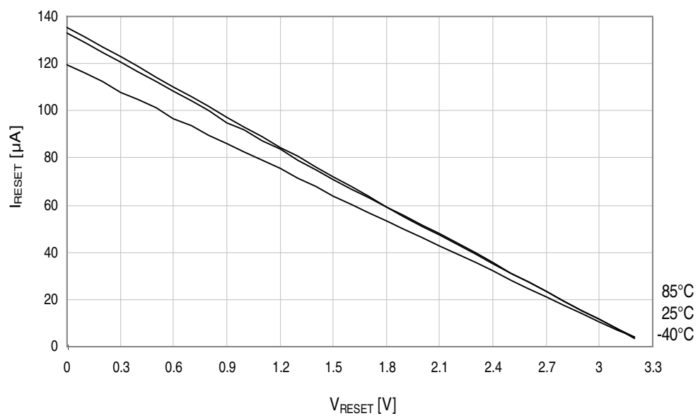
Figure 37-54. Reset pin pull-up resistor current vs. reset pin voltage.
