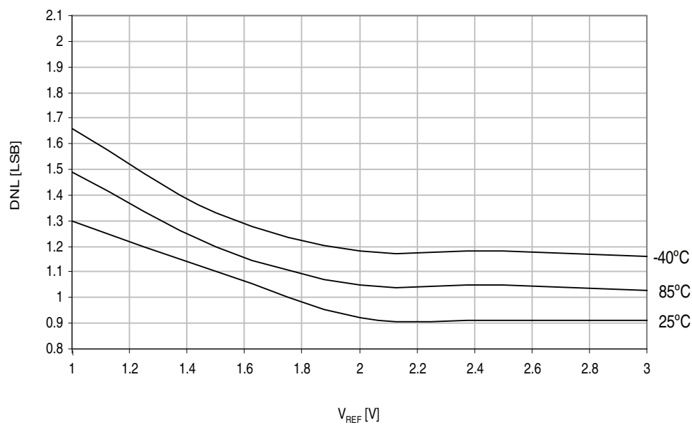
Figure 37-26. ADC DNL vs. V_{REF} . Differential signed mode, V_{CC} = 3.6V , external reference.
