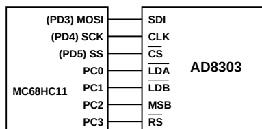
Figure 33. AD8303-MC68HC11 Serial Interface
