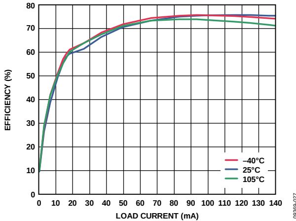
Figure 16. 5 V In to 15 V Out Efficiency over Temperature with Coilcraft Transformer at 500 kHz f_{SW}
