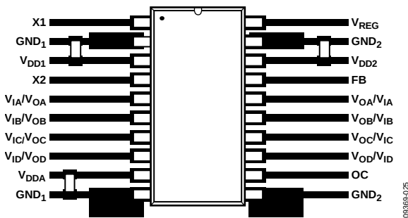
Figure 41. Recommended PCB Layout
