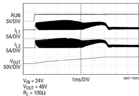
Start-Up
