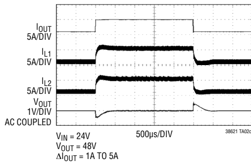
Load Step
