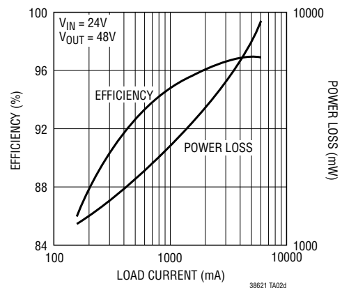
Efficiency
