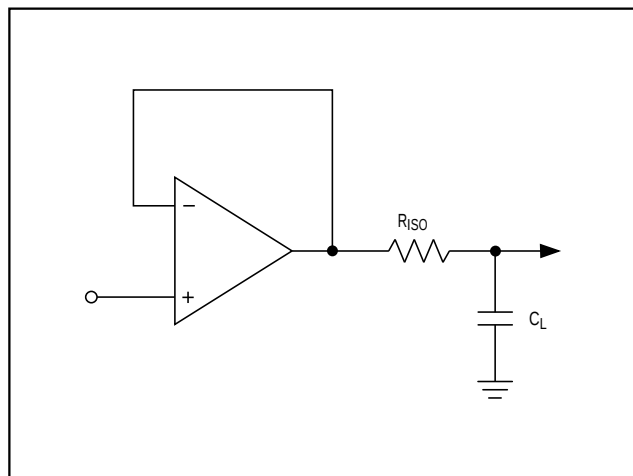
Figure 11. Capacitive-Load-Driving Circuit
