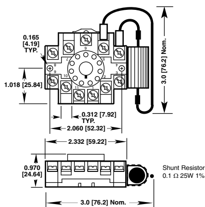
API 011-05A 11-Pin Socket/Shunt 300 V Rating
