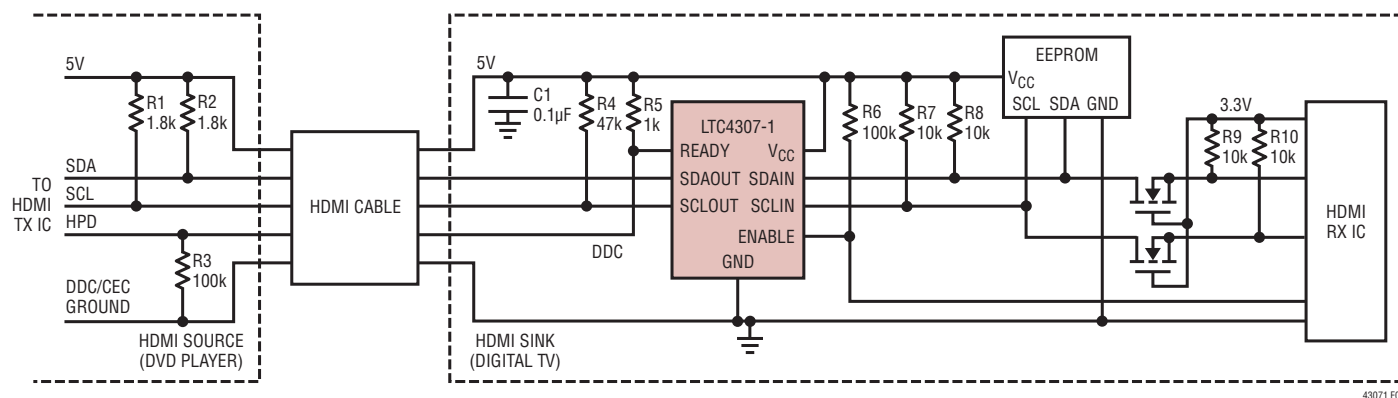
Figure 3. The LTC4307-1 in HDMI Capacitance Buffering Application
