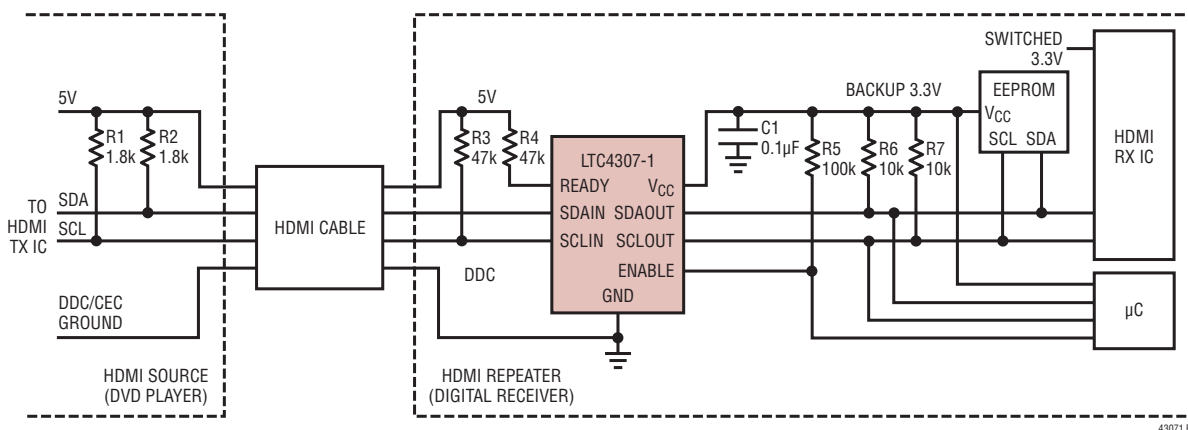
Figure 4. The LTC4307-1 in a Level Shifting and Capacitance Buffering HDMI Application with Backup 3.3V
