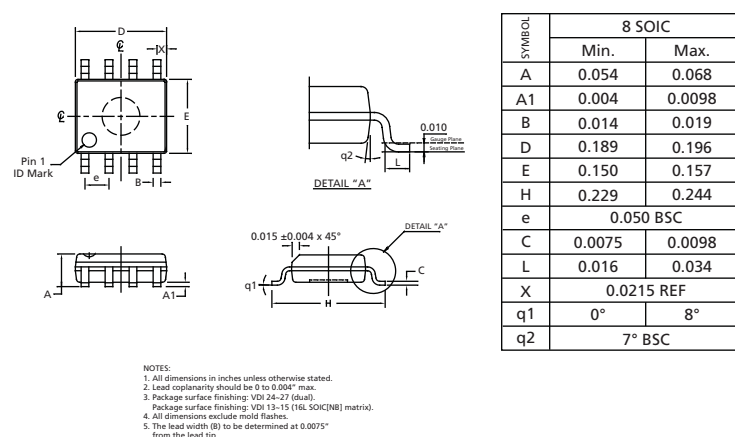
Figure 6-1: Package Dimensions
