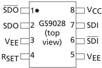
Figure 1-1: Pin Assignment
