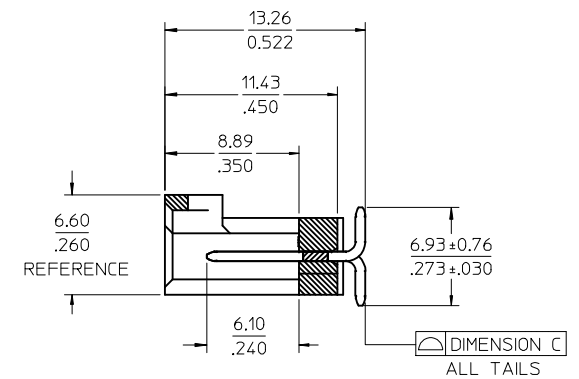
SECTION Z-Z
