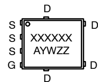
DFN5 & DFNW5 (SO-8FL) CASES 488AA & 507BE
