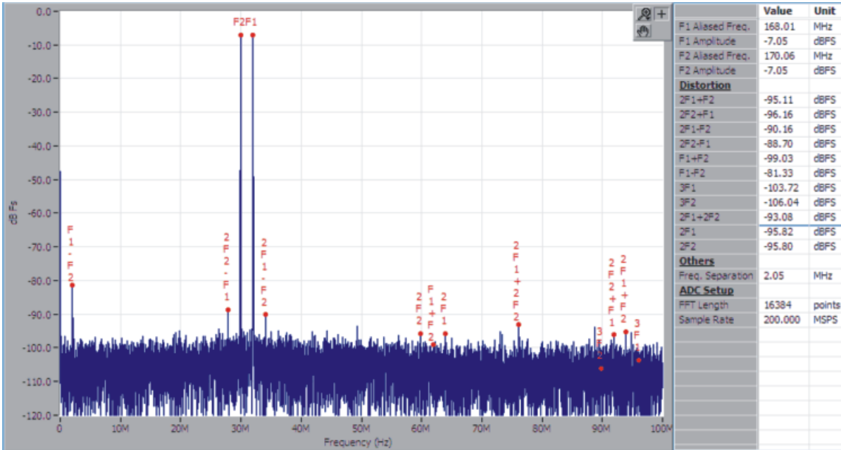
Figure 60. FFT Plot of PGA870 (G = 20 dB) + Second-Order Bandpass Filter and ADS58C48 with Two-Tone Inputs at 168 MHz and 170 MHz
